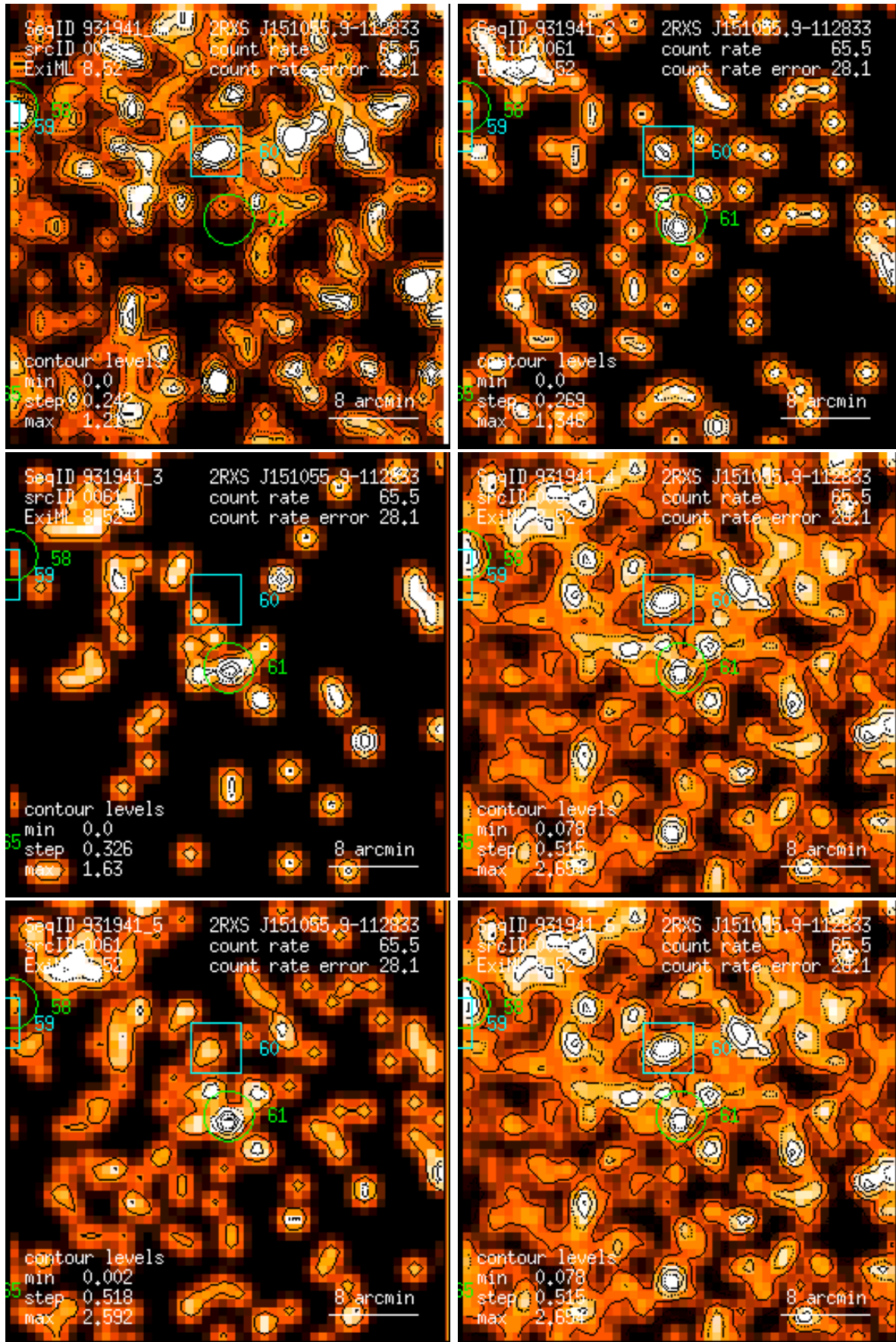
Figure 61: RASS 931941: detection 0061: band rate images, Gaussian filter: (1) PSPC channels 11 – 41, (2) 52 – 90, (3) 91 – 201, (4) 11 – 235, (5) 52 – 201, (6) 11 – 201. Broad band rates in counts/ks. Band rate contour levels in counts/ks/arcmin 2 .
