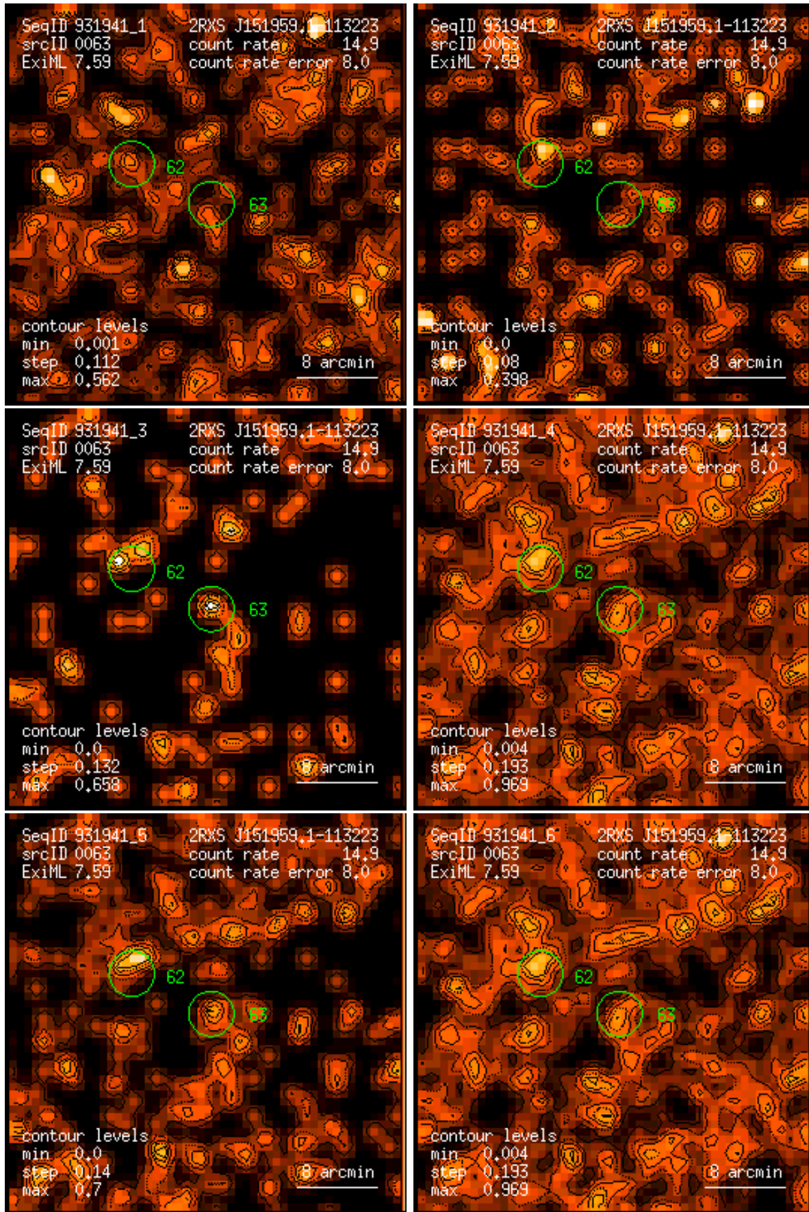
Figure 63: RASS 931941: detection 0063: band rate images, Gaussian filter: (1) PSPC channels 11 – 41, (2) 52 – 90, (3) 91 – 201, (4) 11 – 235, (5) 52 – 201, (6) 11 – 201. Broad band rates in counts/ks. Band rate contour levels in counts/ks/arcmin 2 .
