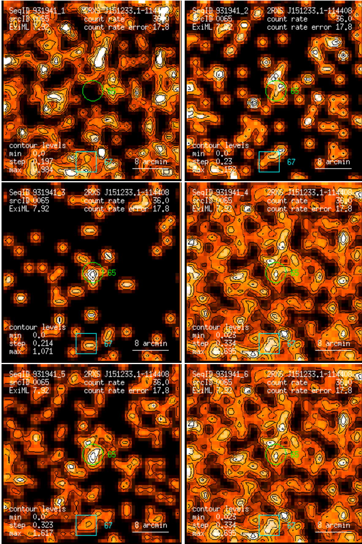
Figure 65: RASS 931941: detection 0065: band rate images, Gaussian filter: (1) PSPC channels 11 – 41, (2) 52 – 90, (3) 91 – 201, (4) 11 – 235, (5) 52 – 201, (6) 11 – 201. Broad band rates in counts/ks. Band rate contour levels in counts/ks/arcmin 2 .
