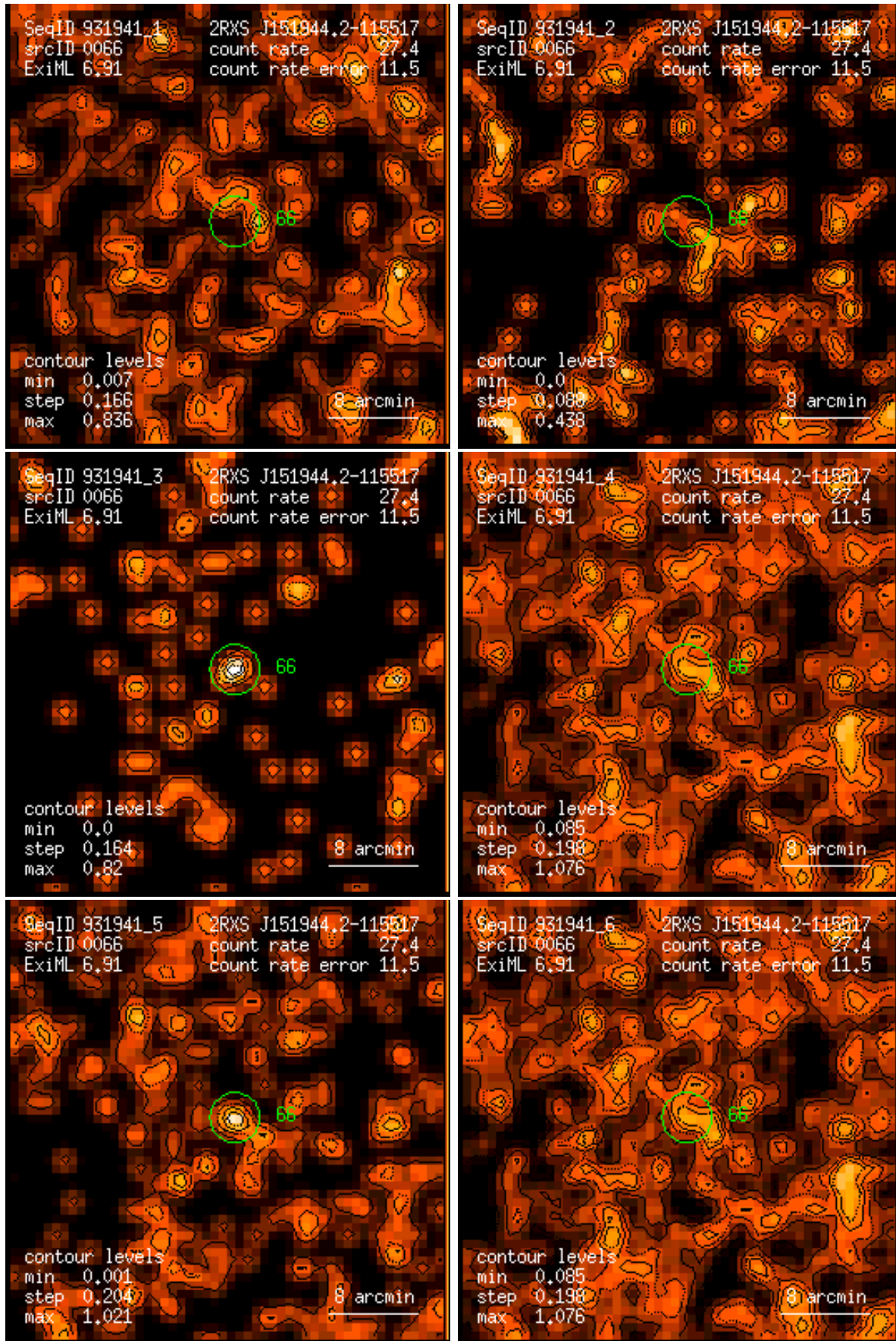
Figure 66: RASS 931941: detection 0066: band rate images, Gaussian filter: (1) PSPC channels 11 – 41, (2) 52 – 90, (3) 91 – 201, (4) 11 – 235, (5) 52 – 201, (6) 11 – 201. Broad band rates in counts/ks. Band rate contour levels in counts/ks/arcmin 2 .
