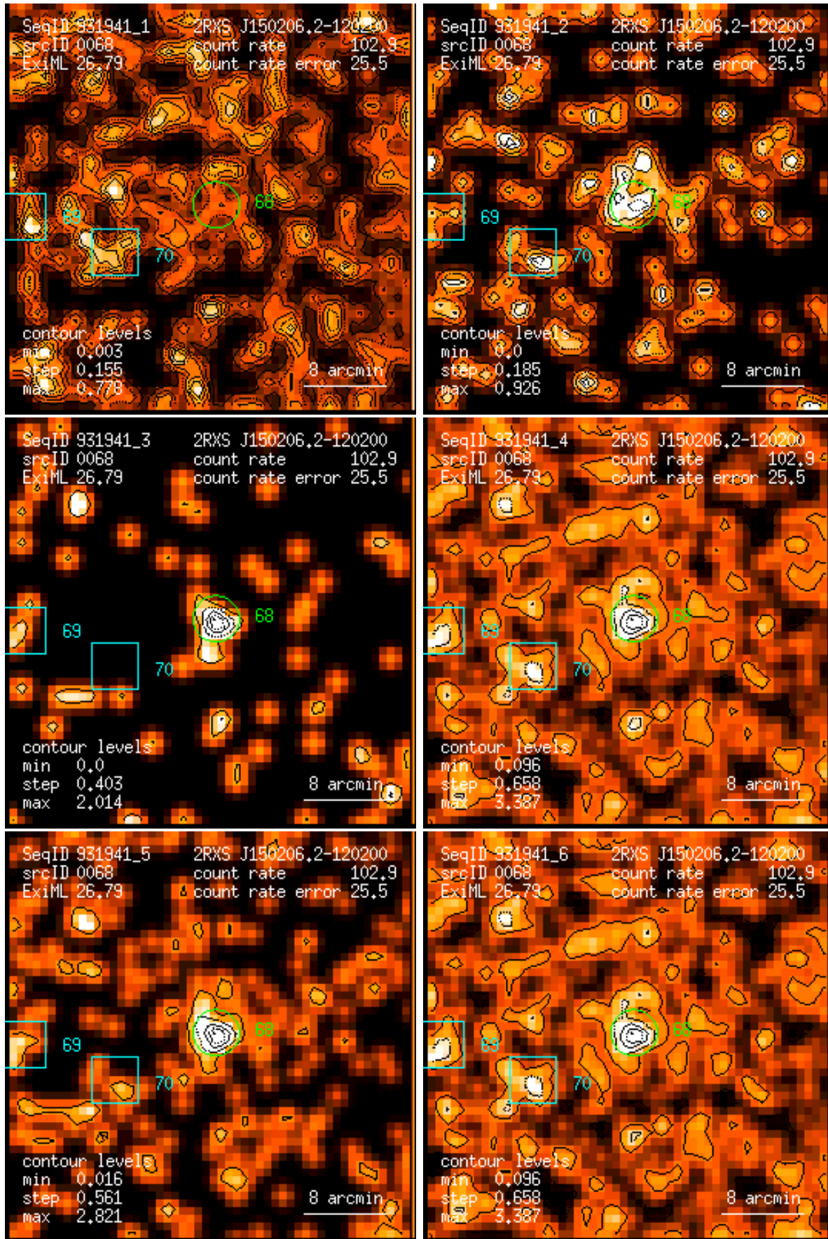
Figure 68: RASS 931941: detection 0068: band rate images, Gaussian filter: (1) PSPC channels 11 – 41, (2) 52 – 90, (3) 91 – 201, (4) 11 – 235, (5) 52 – 201, (6) 11 – 201. Broad band rates in counts/ks. Band rate contour levels in counts/ks/arcmin 2 .
