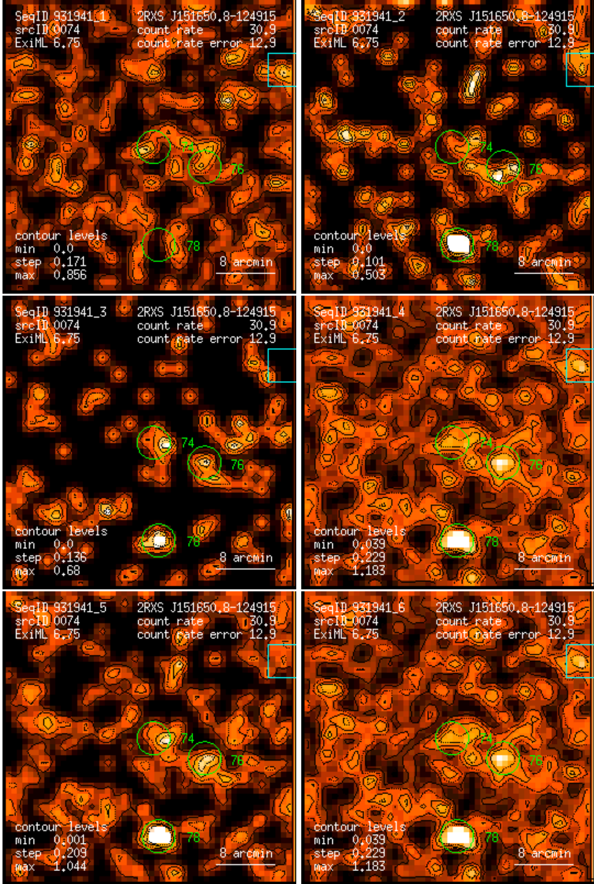
Figure 74: RASS 931941: detection 0074: band rate images, Gaussian filter: (1) PSPC channels 11 – 41, (2) 52 – 90, (3) 91 – 201, (4) 11 – 235, (5) 52 – 201, (6) 11 – 201. Broad band rates in counts/ks. Band rate contour levels in counts/ks/arcmin 2 .
