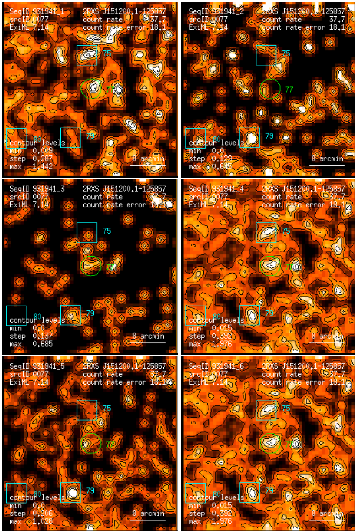
Figure 77: RASS 931941: detection 0077: band rate images, Gaussian filter: (1) PSPC channels 11 – 41, (2) 52 – 90, (3) 91 – 201, (4) 11 – 235, (5) 52 – 201, (6) 11 – 201. Broad band rates in counts/ks. Band rate contour levels in counts/ks/arcmin 2 .
