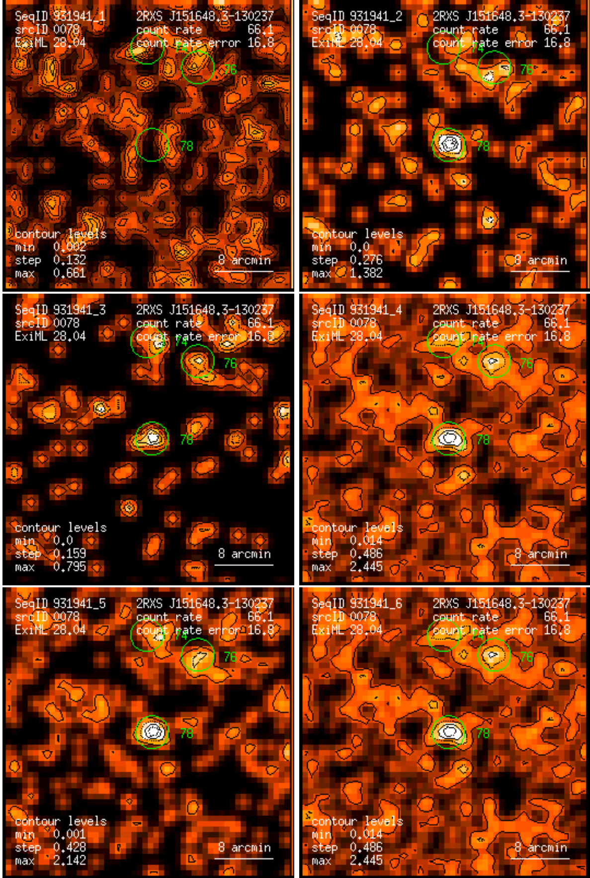
Figure 78: RASS 931941: detection 0078: band rate images, Gaussian filter: (1) PSPC channels 11 – 41, (2) 52 – 90, (3) 91 – 201, (4) 11 – 235, (5) 52 – 201, (6) 11 – 201. Broad band rates in counts/ks. Band rate contour levels in counts/ks/arcmin 2 .
