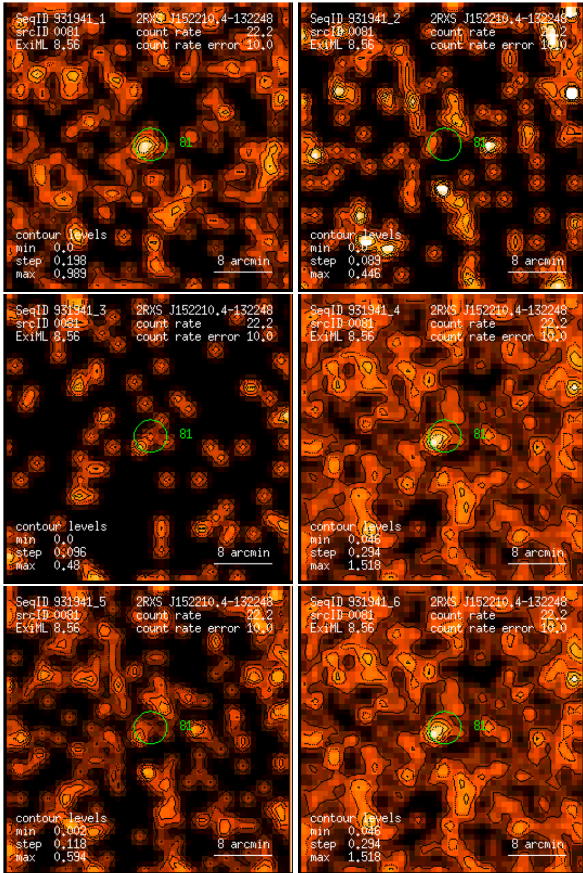
Figure 81: RASS 931941: detection 0081: band rate images, Gaussian filter: (1) PSPC channels 11 – 41, (2) 52 – 90, (3) 91 – 201, (4) 11 – 235, (5) 52 – 201, (6) 11 – 201. Broad band rates in counts/ks. Band rate contour levels in counts/ks/arcmin 2 .
