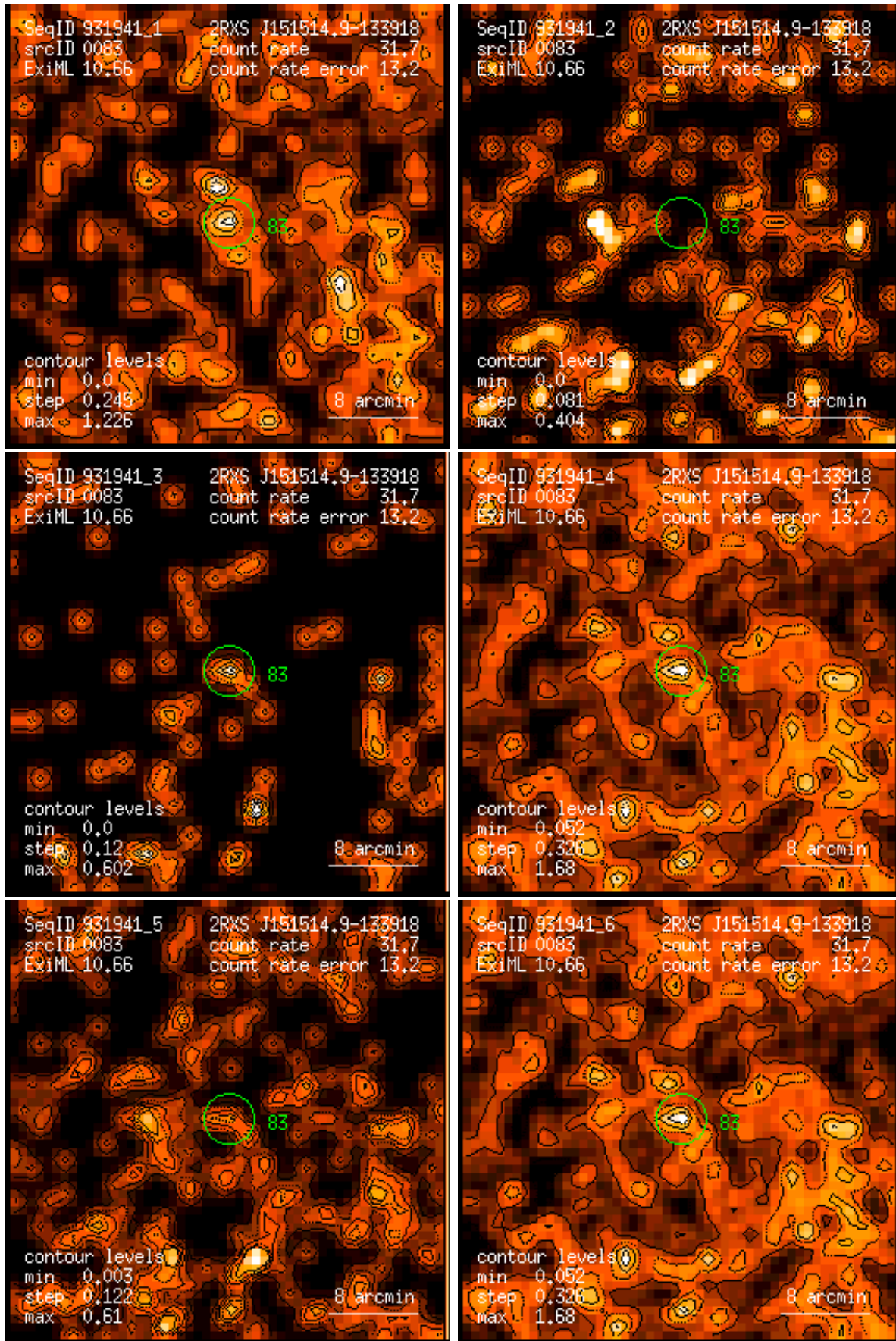
Figure 83: RASS 931941: detection 0083: band rate images, Gaussian filter: (1) PSPC channels 11 – 41, (2) 52 – 90, (3) 91 – 201, (4) 11 – 235, (5) 52 – 201, (6) 11 – 201. Broad band rates in counts/ks. Band rate contour levels in counts/ks/arcmin 2 .
