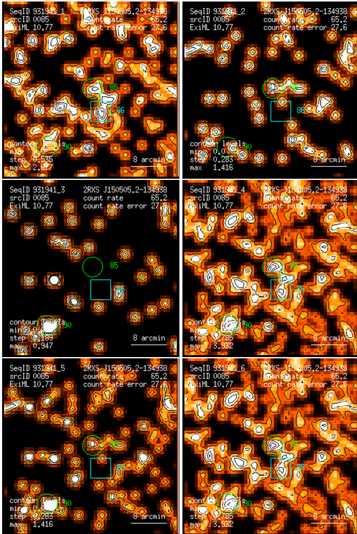
Figure 85: RASS 931941: detection 0085: band rate images, Gaussian filter: (1) PSPC channels 11 – 41, (2) 52 – 90, (3) 91 – 201, (4) 11 – 235, (5) 52 – 201, (6) 11 – 201. Broad band rates in counts/ks. Band rate contour levels in counts/ks/arcmin 2 .
