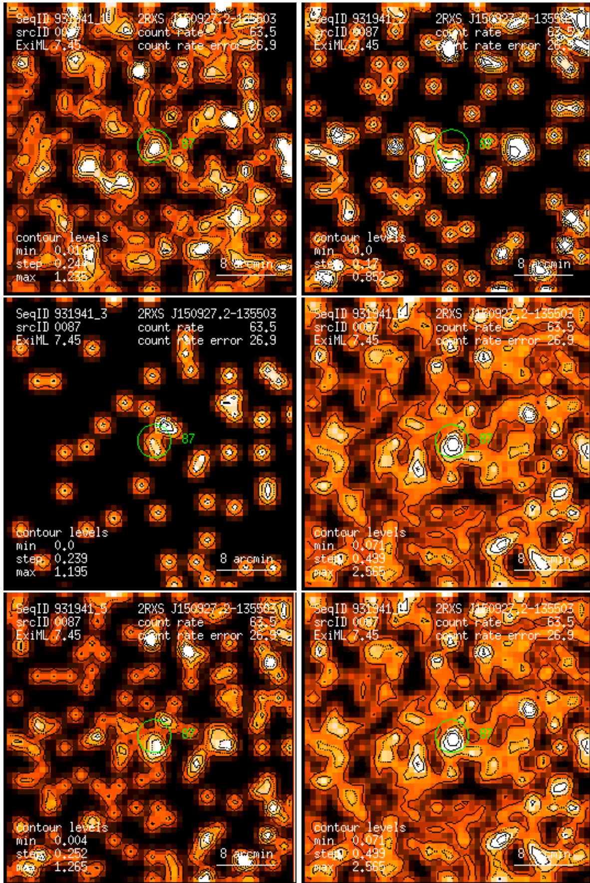
Figure 87: RASS 931941: detection 0087: band rate images, Gaussian filter: (1) PSPC channels 11 – 41, (2) 52 – 90, (3) 91 – 201, (4) 11 – 235, (5) 52 – 201, (6) 11 – 201. Broad band rates in counts/ks. Band rate contour levels in counts/ks/arcmin 2 .
