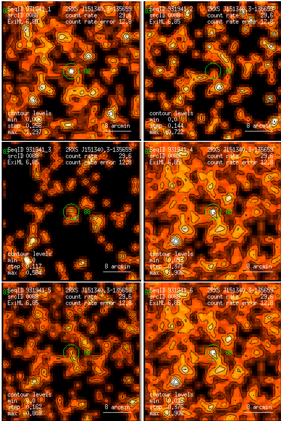
Figure 88: RASS 931941: detection 0088: band rate images, Gaussian filter: (1) PSPC channels 11 – 41, (2) 52 – 90, (3) 91 – 201, (4) 11 – 235, (5) 52 – 201, (6) 11 – 201. Broad band rates in counts/ks. Band rate contour levels in counts/ks/arcmin 2 .
