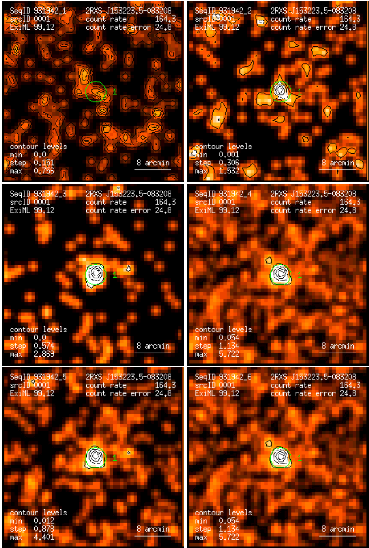
Figure 1: RASS 931942: detection 0001: band rate images, Gaussian filter: (1) PSPC channels 11 – 41, (2) 52 – 90, (3) 91 – 201, (4) 11 – 235, (5) 52 – 201, (6) 11 – 201. Broad band rates in counts/ks. Band rate contour levels in counts/ks/arcmin 2 .
