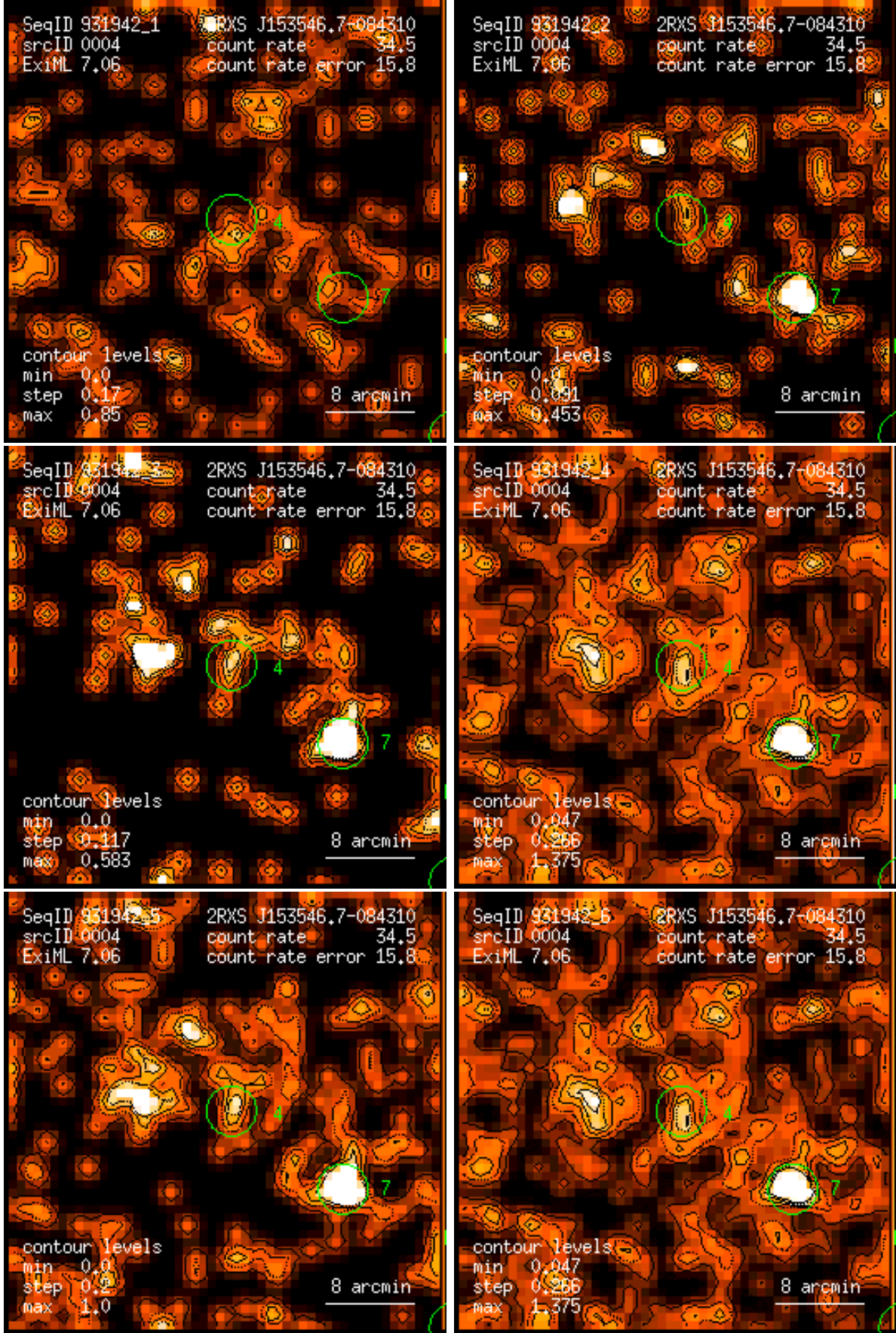
Figure 4: RASS 931942: detection 0004: band rate images, Gaussian filter: (1) PSPC channels 11 – 41, (2) 52 – 90, (3) 91 – 201, (4) 11 – 235, (5) 52 – 201, (6) 11 – 201. Broad band rates in counts/ks. Band rate contour levels in counts/ks/arcmin 2 .
