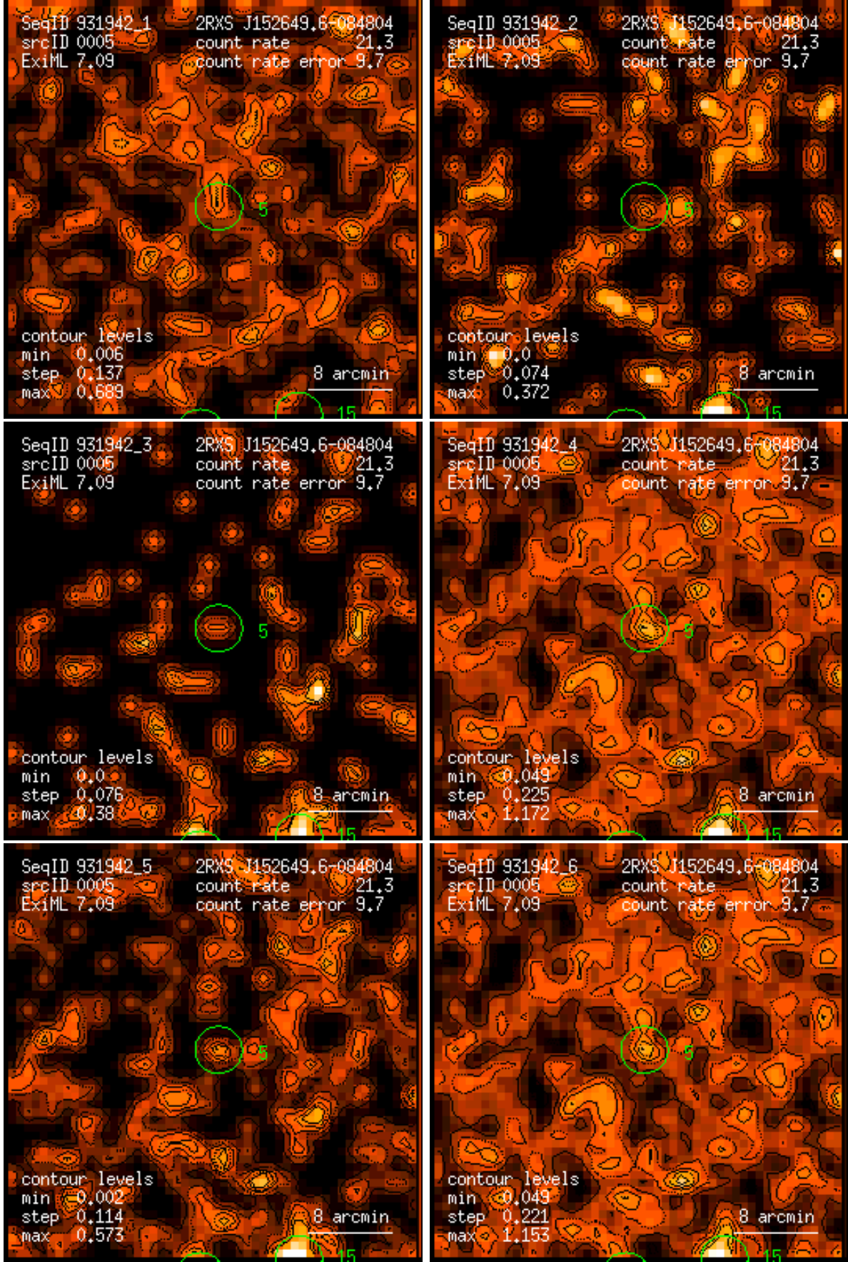
Figure 5: RASS 931942: detection 0005: band rate images, Gaussian filter: (1) PSPC channels 11 – 41, (2) 52 – 90, (3) 91 – 201, (4) 11 – 235, (5) 52 – 201, (6) 11 – 201. Broad band rates in counts/ks. Band rate contour levels in counts/ks/arcmin 2 .
