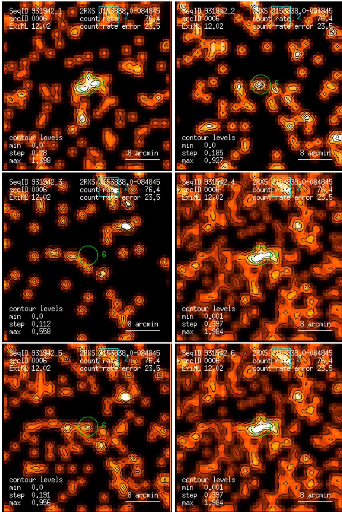
Figure 6: RASS 931942: detection 0006: band rate images, Gaussian filter: (1) PSPC channels 11 – 41, (2) 52 – 90, (3) 91 – 201, (4) 11 – 235, (5) 52 – 201, (6) 11 – 201. Broad band rates in counts/ks. Band rate contour levels in counts/ks/arcmin 2 .
