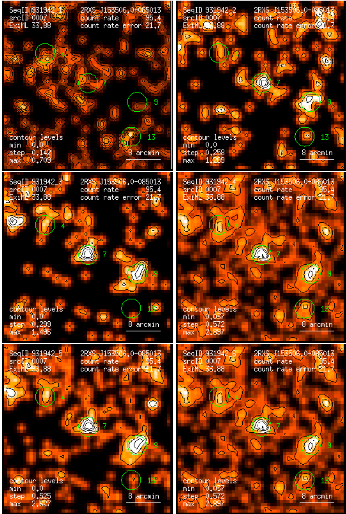
Figure 7: RASS 931942: detection 0007: band rate images, Gaussian filter: (1) PSPC channels 11 – 41, (2) 52 – 90, (3) 91 – 201, (4) 11 – 235, (5) 52 – 201, (6) 11 – 201. Broad band rates in counts/ks. Band rate contour levels in counts/ks/arcmin 2 .
