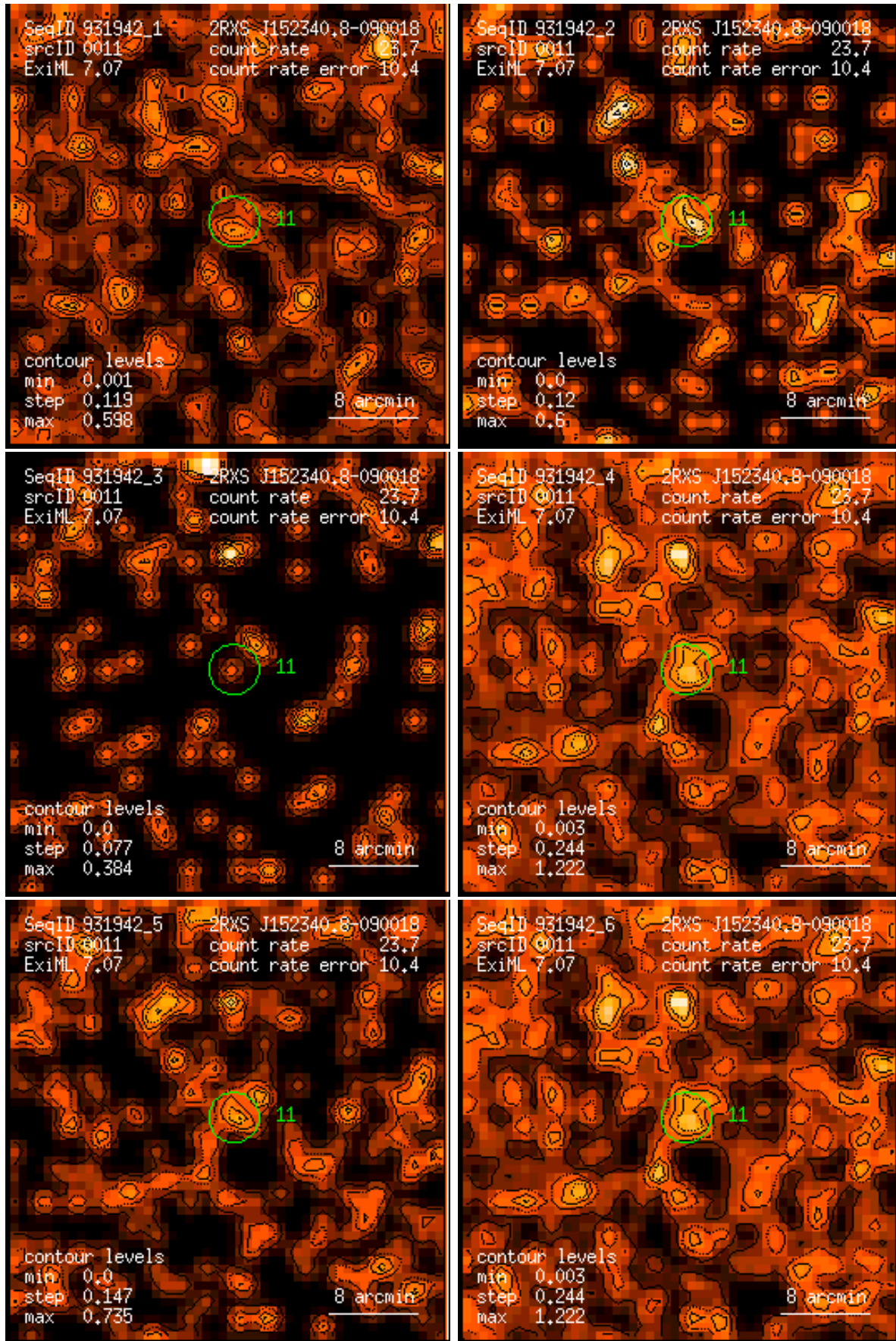
Figure 11: RASS 931942: detection 0011: band rate images, Gaussian filter: (1) PSPC channels 11 – 41, (2) 52 – 90, (3) 91 – 201, (4) 11 – 235, (5) 52 – 201, (6) 11 – 201. Broad band rates in counts/ks. Band rate contour levels in counts/ks/arcmin 2 .
