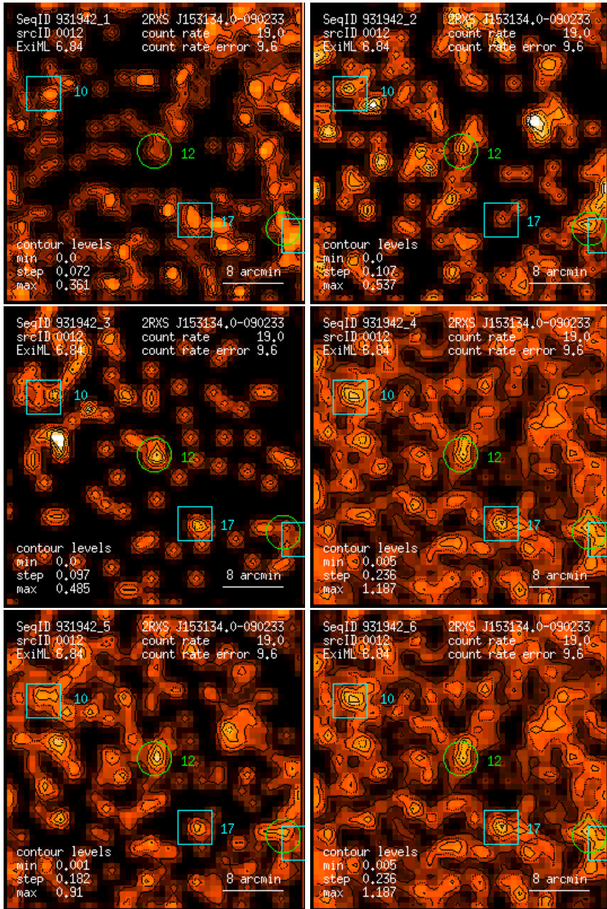
Figure 12: RASS 931942: detection 0012: band rate images, Gaussian filter: (1) PSPC channels 11 – 41, (2) 52 – 90, (3) 91 – 201, (4) 11 – 235, (5) 52 – 201, (6) 11 – 201. Broad band rates in counts/ks. Band rate contour levels in counts/ks/arcmin 2 .
