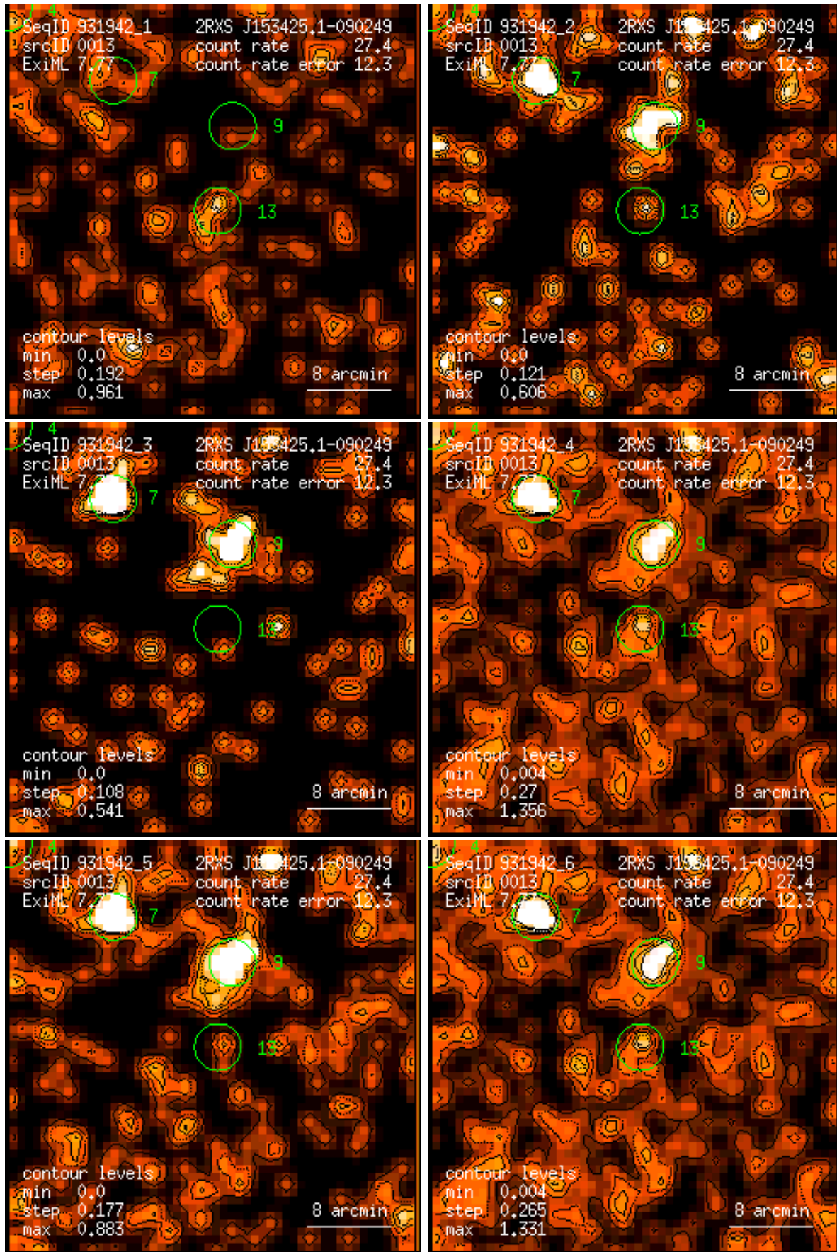
Figure 13: RASS 931942: detection 0013: band rate images, Gaussian filter: (1) PSPC channels 11 – 41, (2) 52 – 90, (3) 91 – 201, (4) 11 – 235, (5) 52 – 201, (6) 11 – 201. Broad band rates in counts/ks. Band rate contour levels in counts/ks/arcmin 2 .
