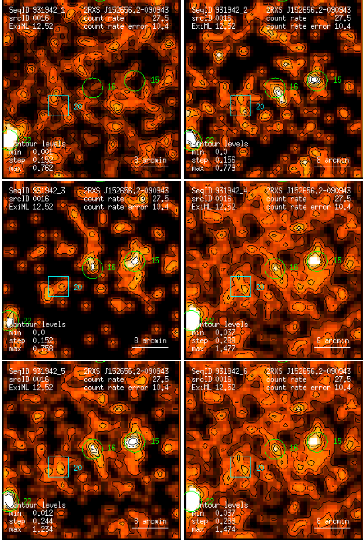
Figure 16: RASS 931942: detection 0016: band rate images, Gaussian filter: (1) PSPC channels 11 – 41, (2) 52 – 90, (3) 91 – 201, (4) 11 – 235, (5) 52 – 201, (6) 11 – 201. Broad band rates in counts/ks. Band rate contour levels in counts/ks/arcmin 2 .
