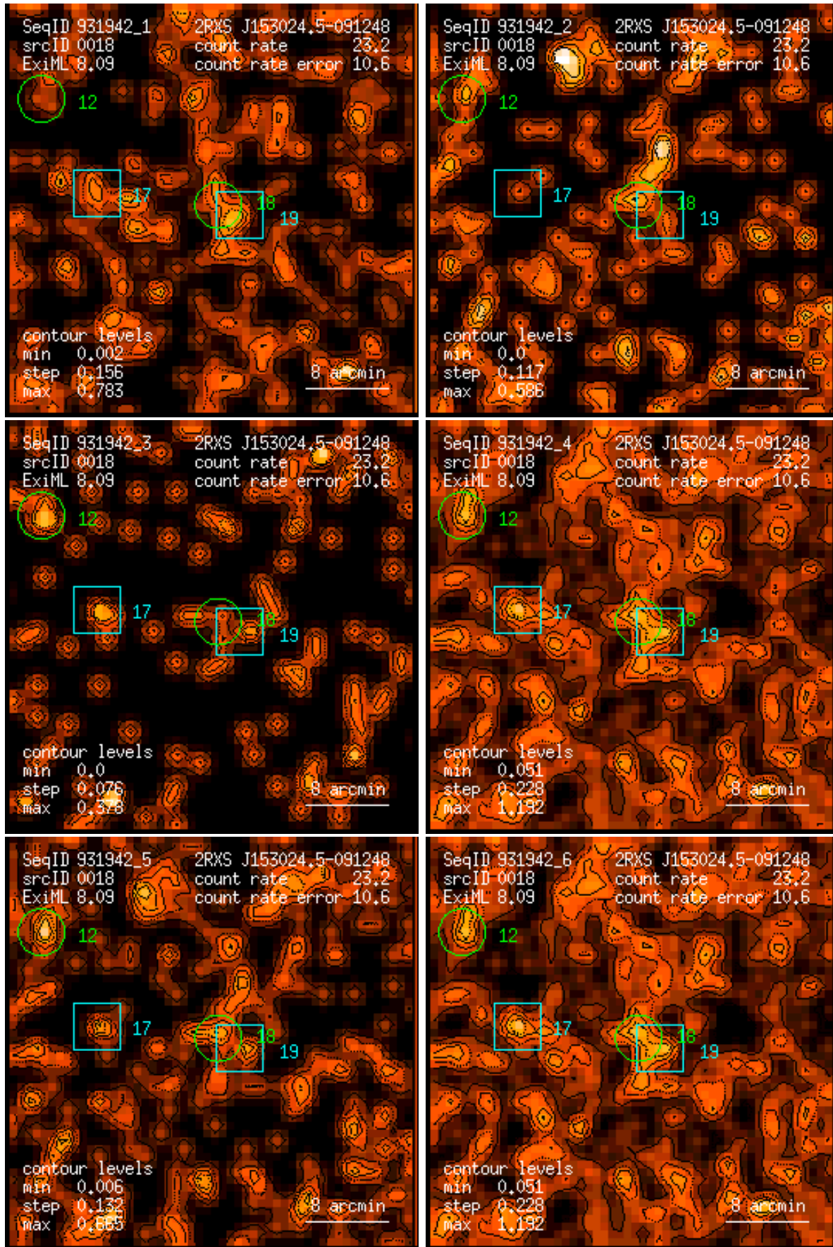
Figure 18: RASS 931942: detection 0018: band rate images, Gaussian filter: (1) PSPC channels 11 – 41, (2) 52 – 90, (3) 91 – 201, (4) 11 – 235, (5) 52 – 201, (6) 11 – 201. Broad band rates in counts/ks. Band rate contour levels in counts/ks/arcmin 2 .
