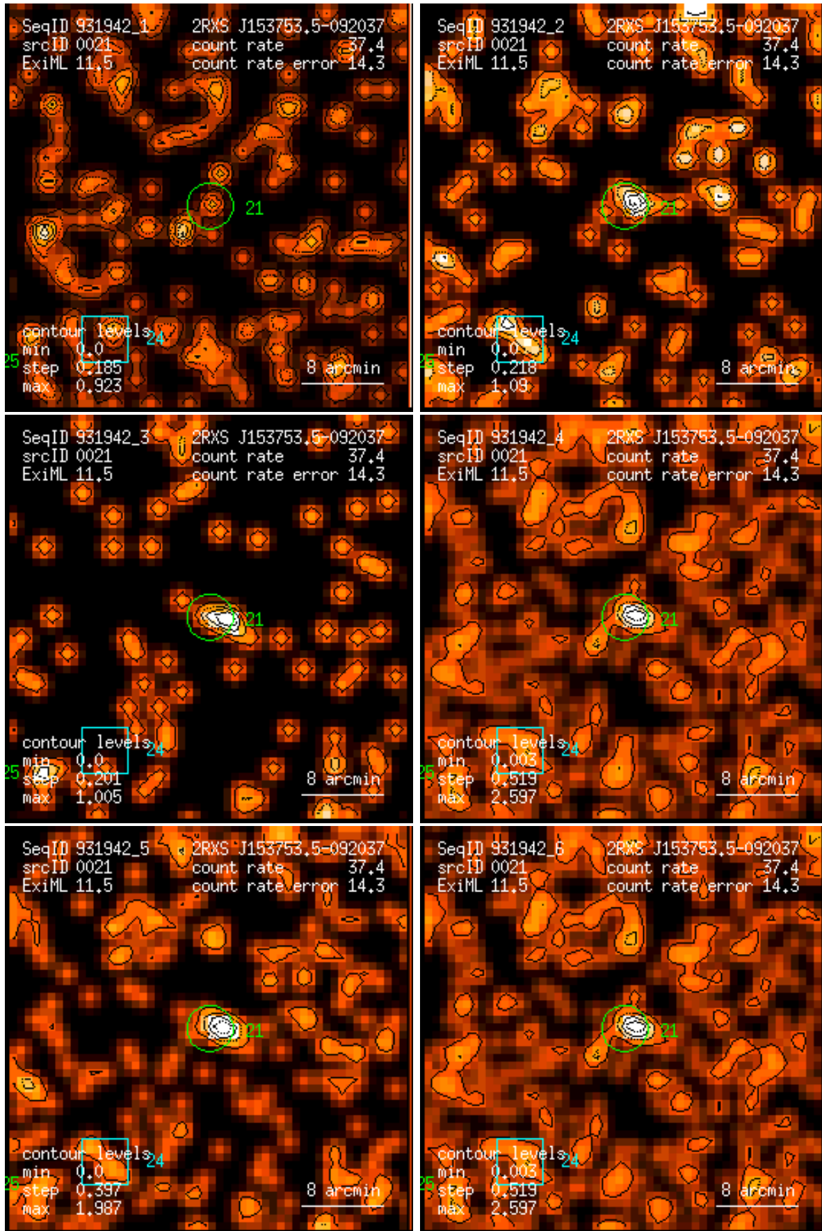
Figure 21: RASS 931942: detection 0021: band rate images, Gaussian filter: (1) PSPC channels 11 – 41, (2) 52 – 90, (3) 91 – 201, (4) 11 – 235, (5) 52 – 201, (6) 11 – 201. Broad band rates in counts/ks. Band rate contour levels in counts/ks/arcmin 2 .
