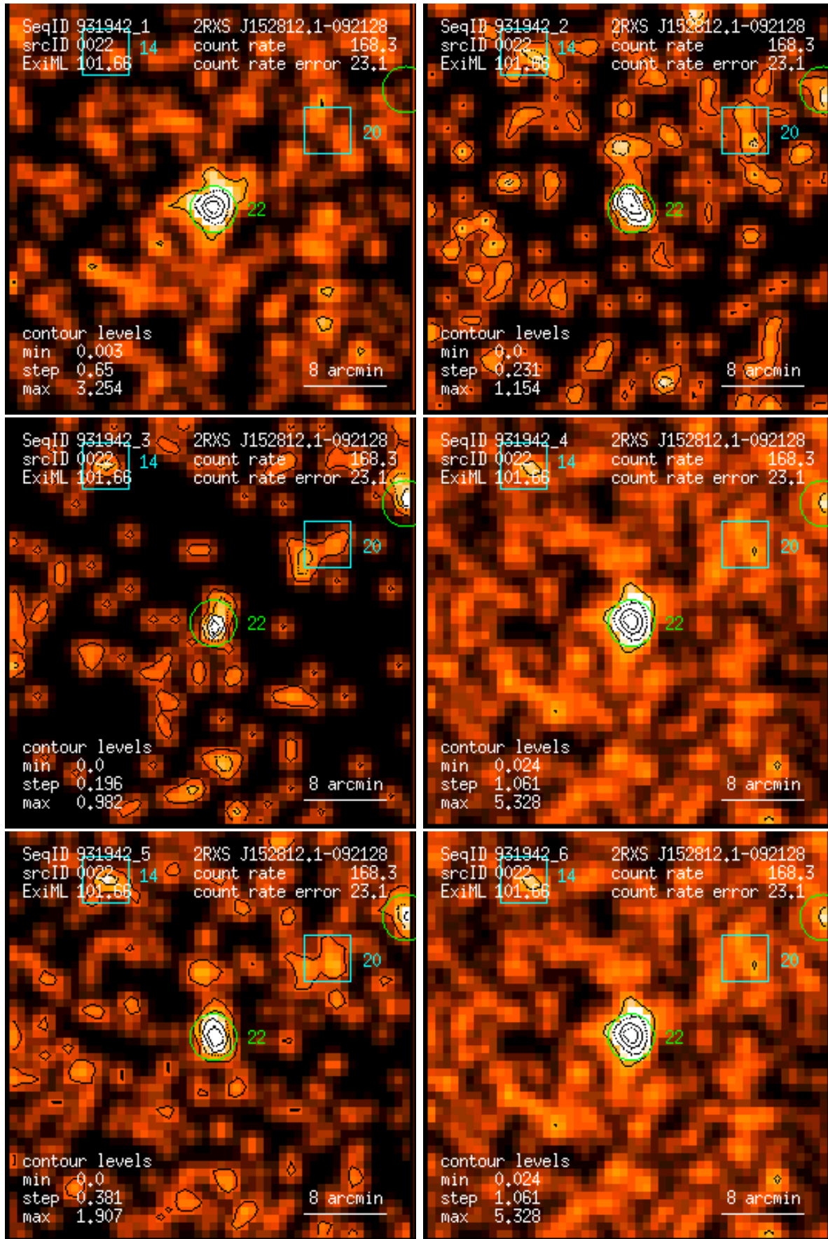
Figure 22: RASS 931942: detection 0022: band rate images, Gaussian filter: (1) PSPC channels 11 – 41, (2) 52 – 90, (3) 91 – 201, (4) 11 – 235, (5) 52 – 201, (6) 11 – 201. Broad band rates in counts/ks. Band rate contour levels in counts/ks/arcmin 2 .
