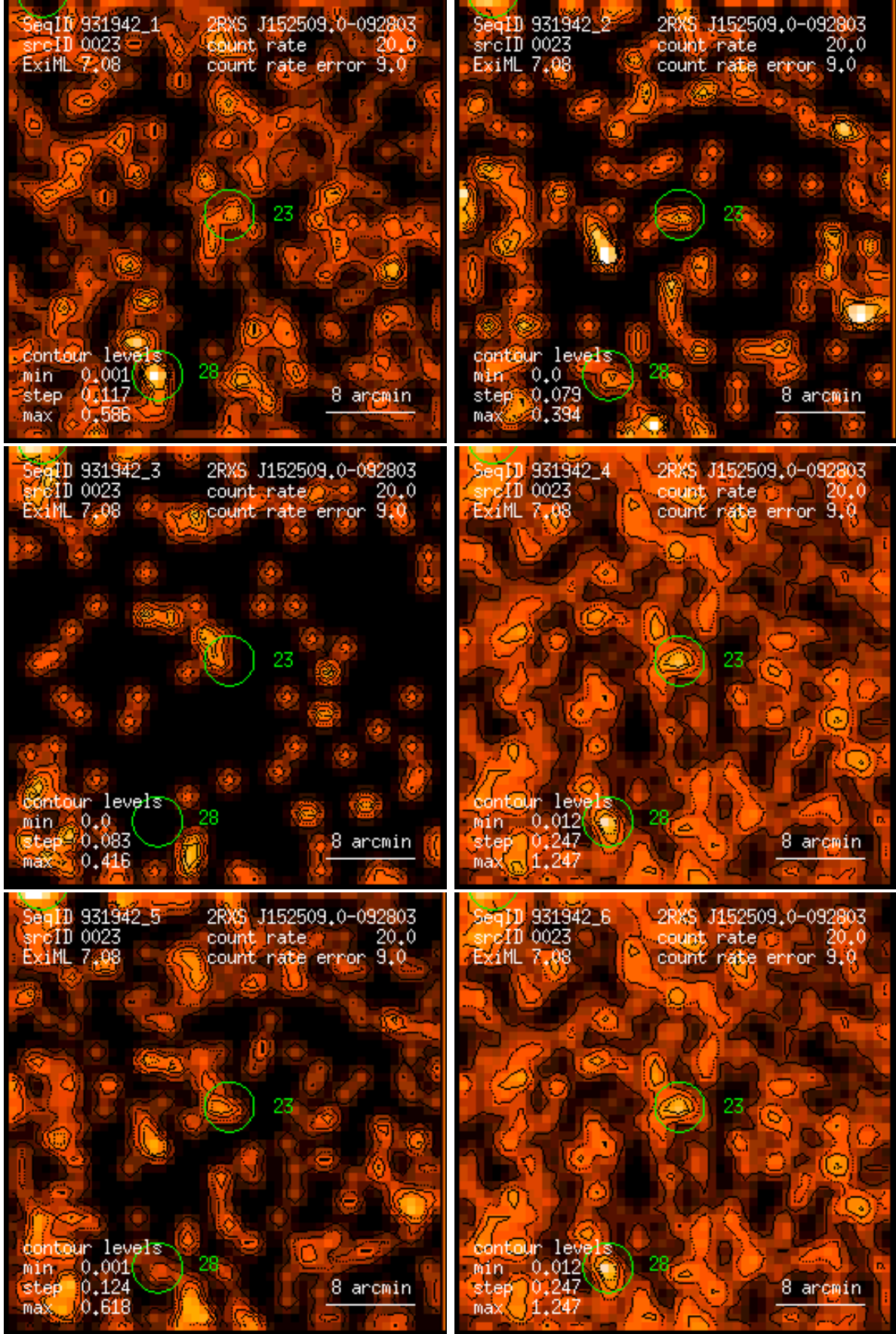
Figure 23: RASS 931942: detection 0023: band rate images, Gaussian filter: (1) PSPC channels 11 – 41, (2) 52 – 90, (3) 91 – 201, (4) 11 – 235, (5) 52 – 201, (6) 11 – 201. Broad band rates in counts/ks. Band rate contour levels in counts/ks/arcmin 2 .
