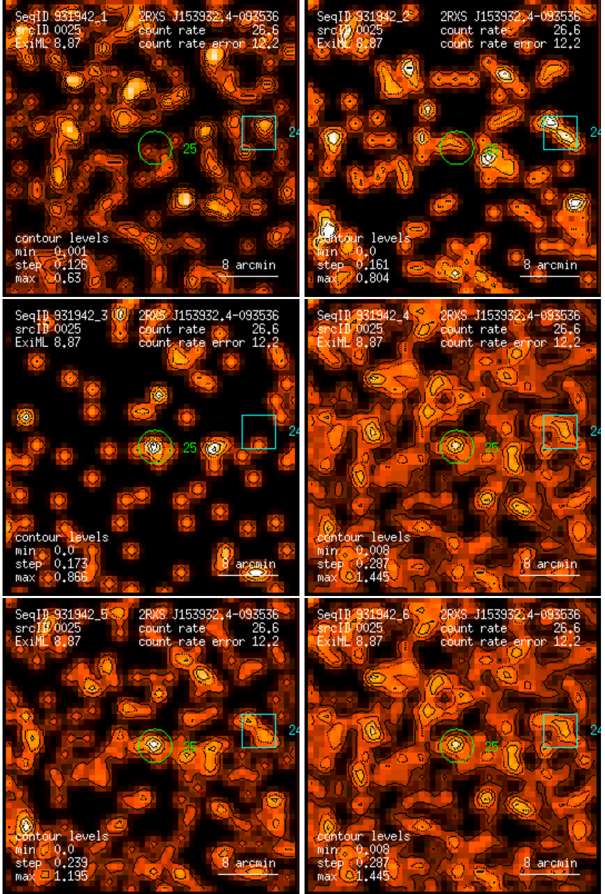
Figure 25: RASS 931942: detection 0025: band rate images, Gaussian filter: (1) PSPC channels 11 – 41, (2) 52 – 90, (3) 91 – 201, (4) 11 – 235, (5) 52 – 201, (6) 11 – 201. Broad band rates in counts/ks. Band rate contour levels in counts/ks/arcmin 2 .
