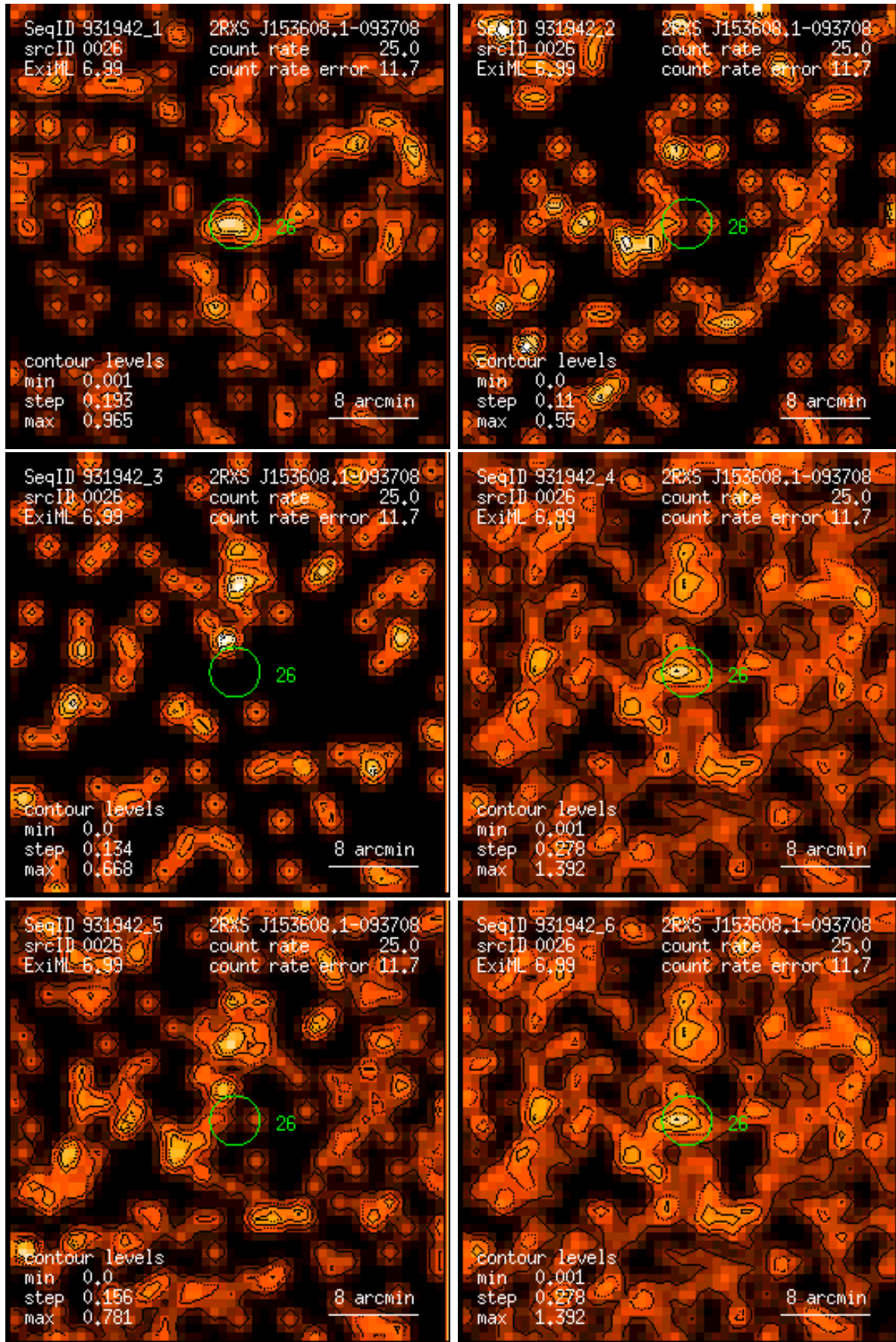
Figure 26: RASS 931942: detection 0026: band rate images, Gaussian filter: (1) PSPC channels 11 – 41, (2) 52 – 90, (3) 91 – 201, (4) 11 – 235, (5) 52 – 201, (6) 11 – 201. Broad band rates in counts/ks. Band rate contour levels in counts/ks/arcmin 2 .
