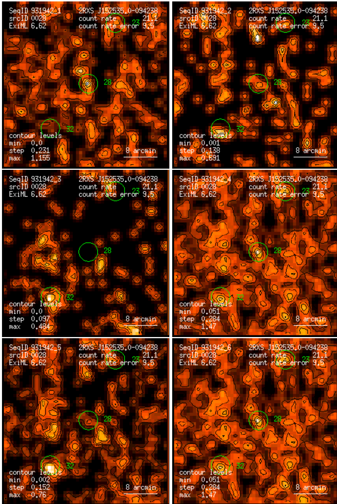
Figure 28: RASS 931942: detection 0028: band rate images, Gaussian filter: (1) PSPC channels 11 – 41, (2) 52 – 90, (3) 91 – 201, (4) 11 – 235, (5) 52 – 201, (6) 11 – 201. Broad band rates in counts/ks. Band rate contour levels in counts/ks/arcmin 2 .
