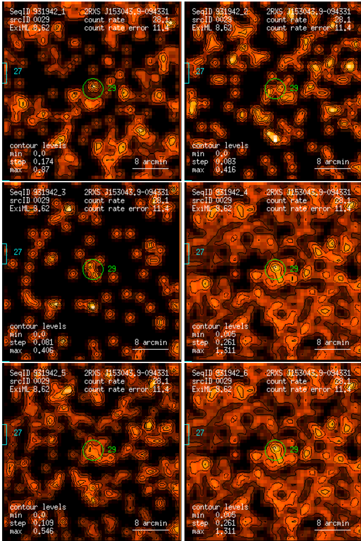
Figure 29: RASS 931942: detection 0029: band rate images, Gaussian filter: (1) PSPC channels 11 – 41, (2) 52 – 90, (3) 91 – 201, (4) 11 – 235, (5) 52 – 201, (6) 11 – 201. Broad band rates in counts/ks. Band rate contour levels in counts/ks/arcmin 2 .
