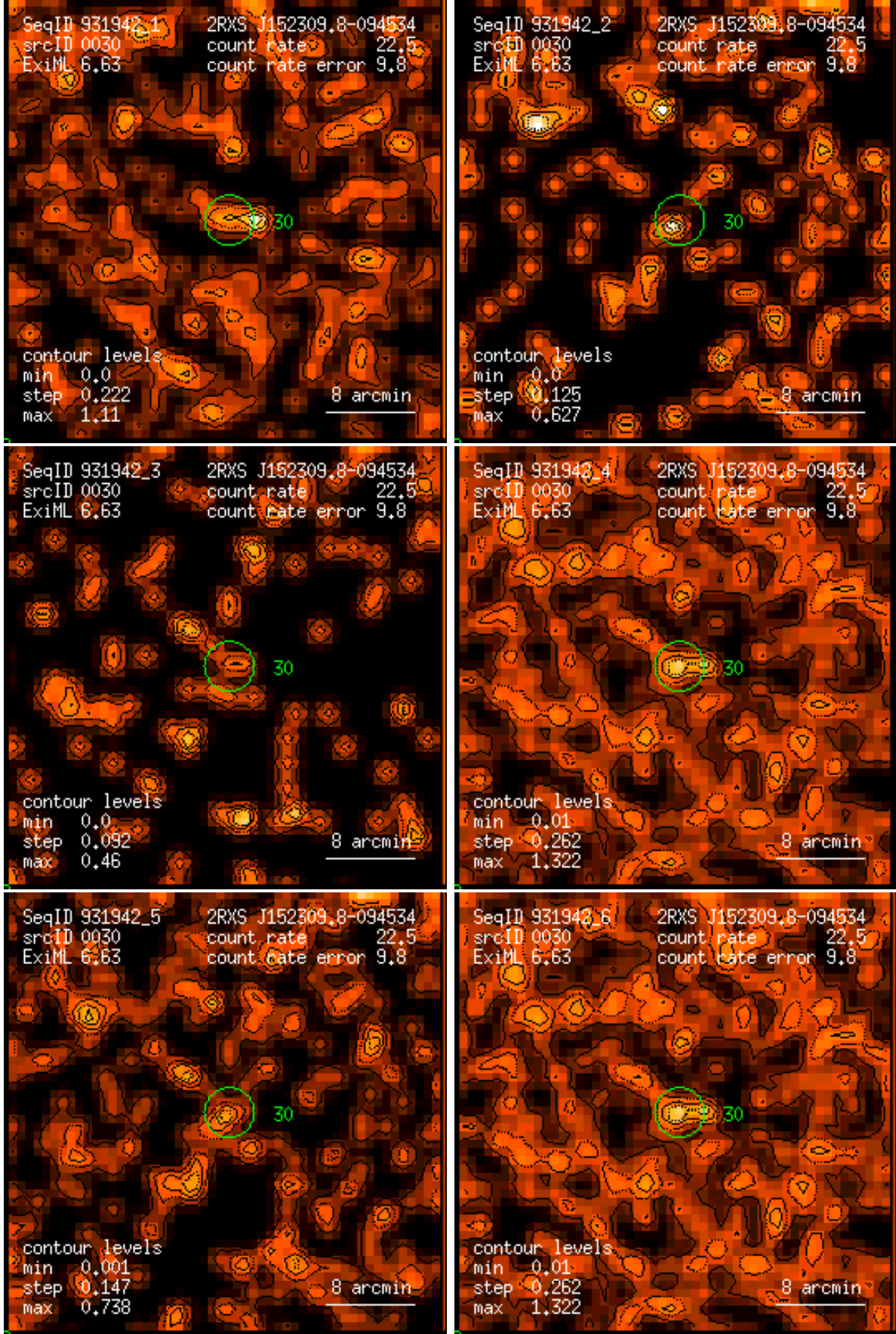
Figure 30: RASS 931942: detection 0030: band rate images, Gaussian filter: (1) PSPC channels 11 – 41, (2) 52 – 90, (3) 91 – 201, (4) 11 – 235, (5) 52 – 201, (6) 11 – 201. Broad band rates in counts/ks. Band rate contour levels in counts/ks/arcmin 2 .
