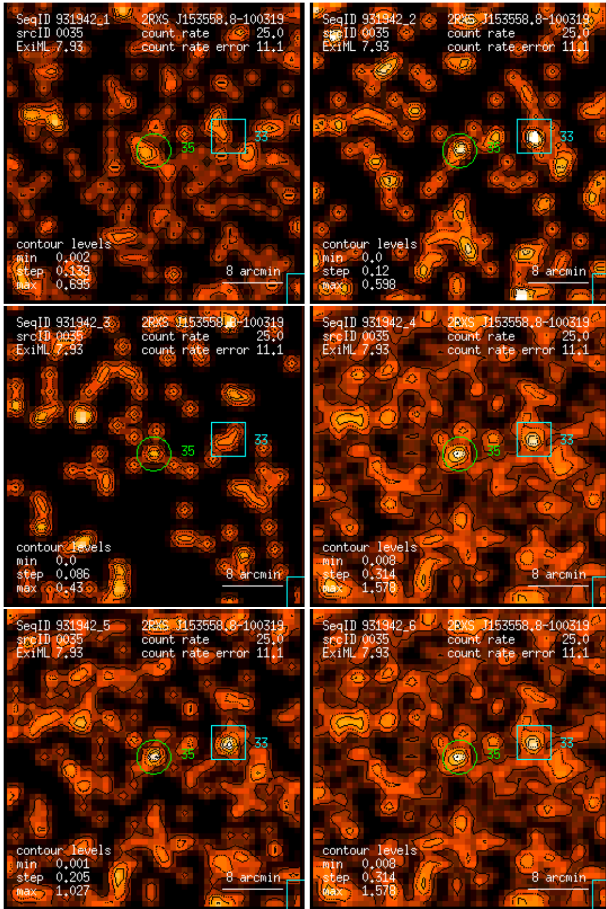
Figure 35: RASS 931942: detection 0035: band rate images, Gaussian filter: (1) PSPC channels 11 – 41, (2) 52 – 90, (3) 91 – 201, (4) 11 – 235, (5) 52 – 201, (6) 11 – 201. Broad band rates in counts/ks. Band rate contour levels in counts/ks/arcmin 2 .
