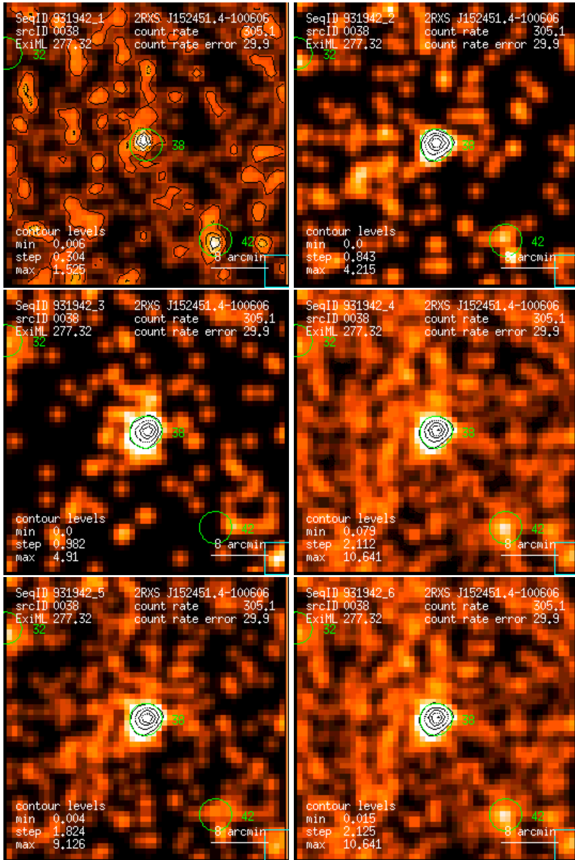
Figure 38: RASS 931942: detection 0038: band rate images, Gaussian filter: (1) PSPC channels 11 – 41, (2) 52 – 90, (3) 91 – 201, (4) 11 – 235, (5) 52 – 201, (6) 11 – 201. Broad band rates in counts/ks. Band rate contour levels in counts/ks/arcmin 2 .
