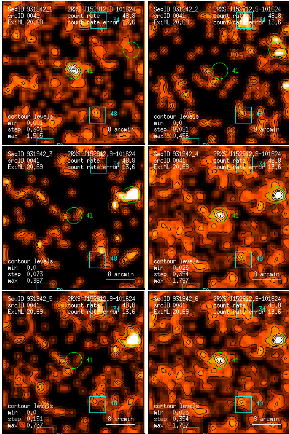
Figure 41: RASS 931942: detection 0041: band rate images, Gaussian filter: (1) PSPC channels 11 – 41, (2) 52 – 90, (3) 91 – 201, (4) 11 – 235, (5) 52 – 201, (6) 11 – 201. Broad band rates in counts/ks. Band rate contour levels in counts/ks/arcmin 2 .
