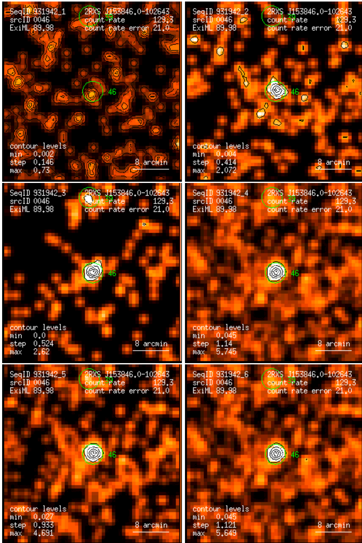
Figure 46: RASS 931942: detection 0046: band rate images, Gaussian filter: (1) PSPC channels 11 – 41, (2) 52 – 90, (3) 91 – 201, (4) 11 – 235, (5) 52 – 201, (6) 11 – 201. Broad band rates in counts/ks. Band rate contour levels in counts/ks/arcmin 2 .
