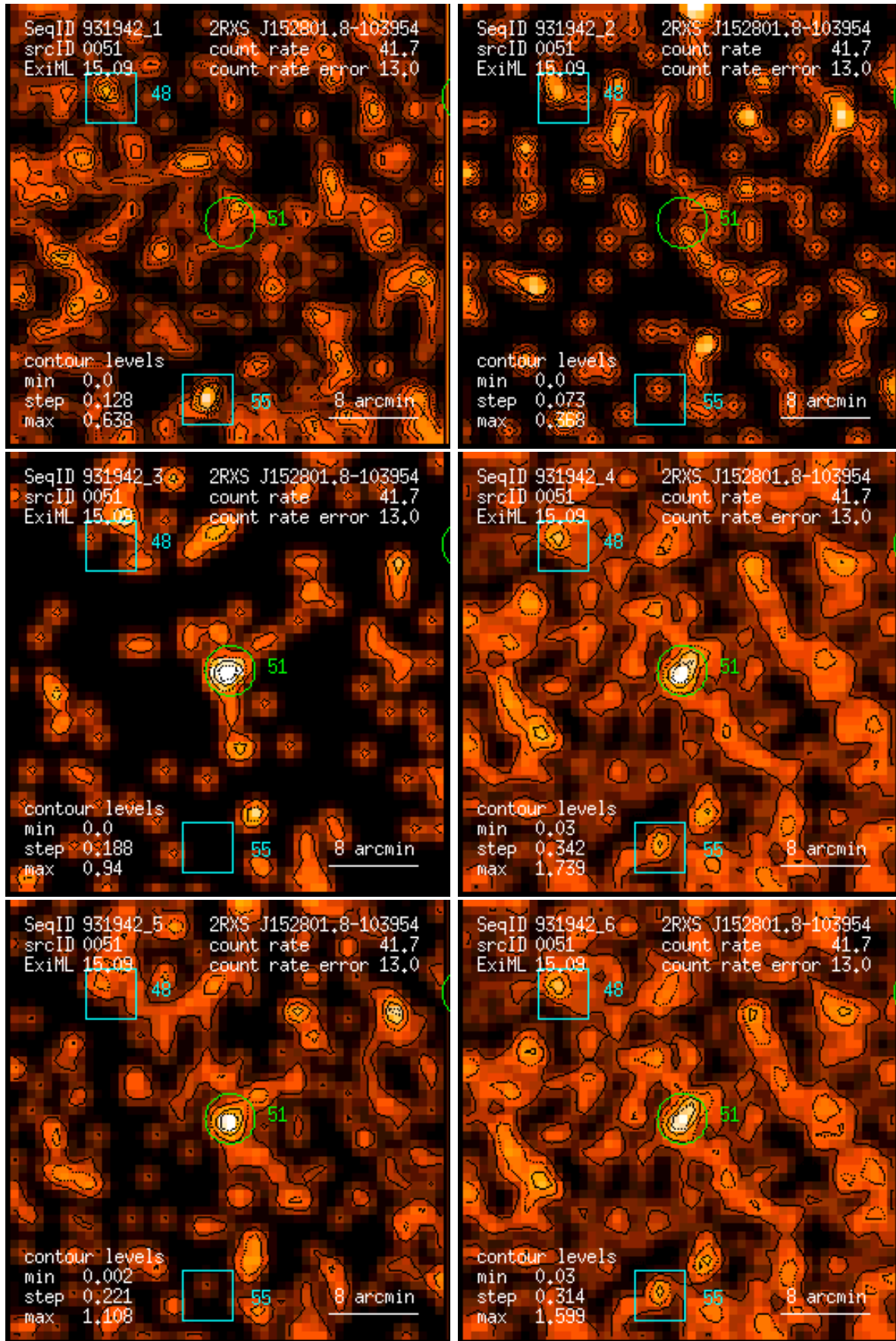
Figure 51: RASS 931942: detection 0051: band rate images, Gaussian filter: (1) PSPC channels 11 – 41, (2) 52 – 90, (3) 91 – 201, (4) 11 – 235, (5) 52 – 201, (6) 11 – 201. Broad band rates in counts/ks. Band rate contour levels in counts/ks/arcmin 2 .
