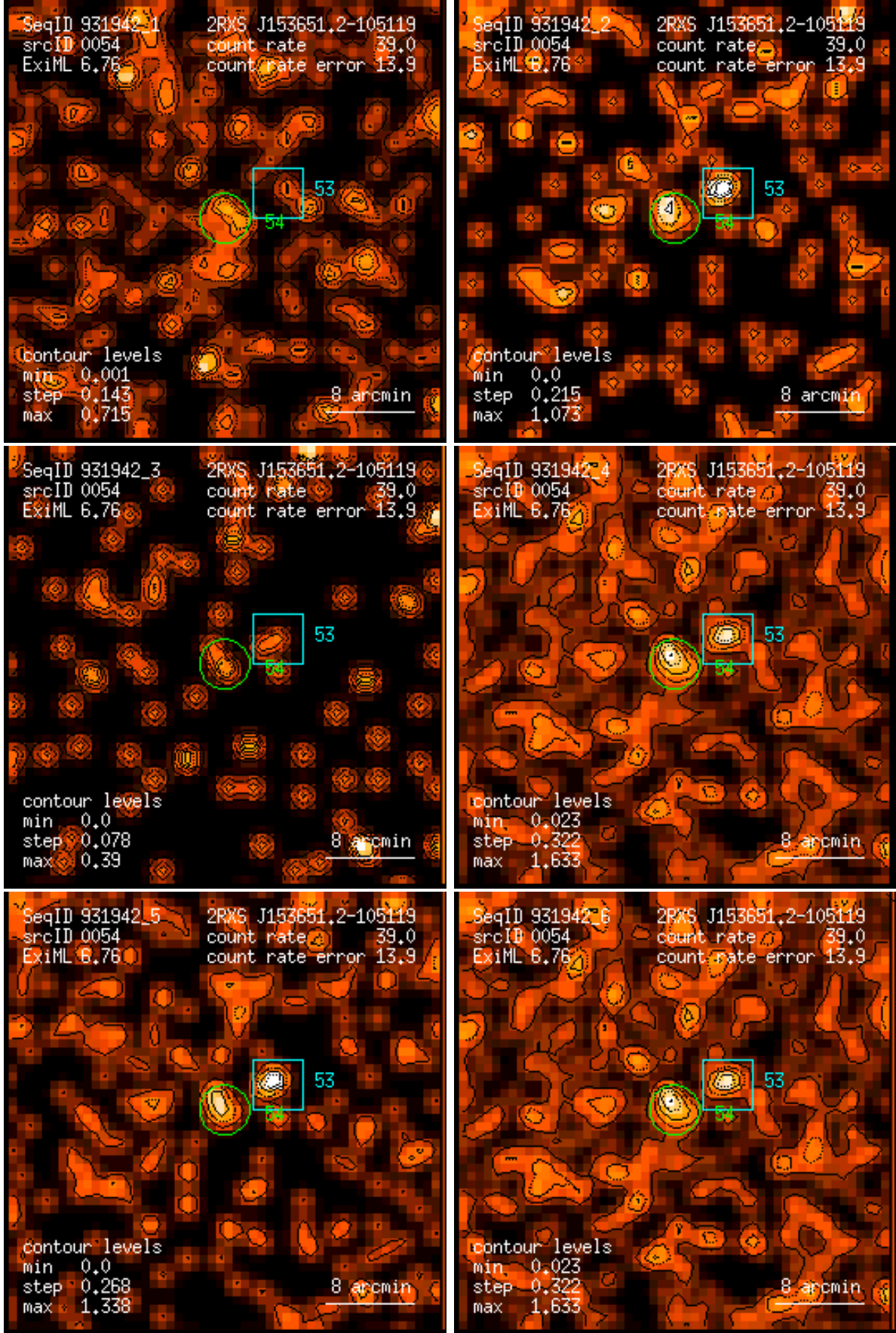
Figure 54: RASS 931942: detection 0054: band rate images, Gaussian filter: (1) PSPC channels 11 – 41, (2) 52 – 90, (3) 91 – 201, (4) 11 – 235, (5) 52 – 201, (6) 11 – 201. Broad band rates in counts/ks. Band rate contour levels in counts/ks/arcmin 2 .
