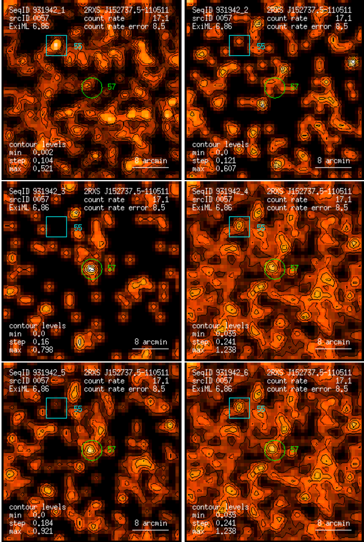
Figure 57: RASS 931942: detection 0057: band rate images, Gaussian filter: (1) PSPC channels 11 – 41, (2) 52 – 90, (3) 91 – 201, (4) 11 – 235, (5) 52 – 201, (6) 11 – 201. Broad band rates in counts/ks. Band rate contour levels in counts/ks/arcmin 2 .
