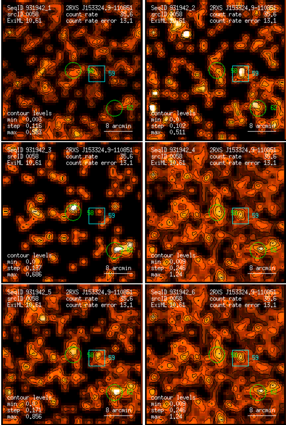
Figure 58: RASS 931942: detection 0058: band rate images, Gaussian filter: (1) PSPC channels 11 – 41, (2) 52 – 90, (3) 91 – 201, (4) 11 – 235, (5) 52 – 201, (6) 11 – 201. Broad band rates in counts/ks. Band rate contour levels in counts/ks/arcmin 2 .
