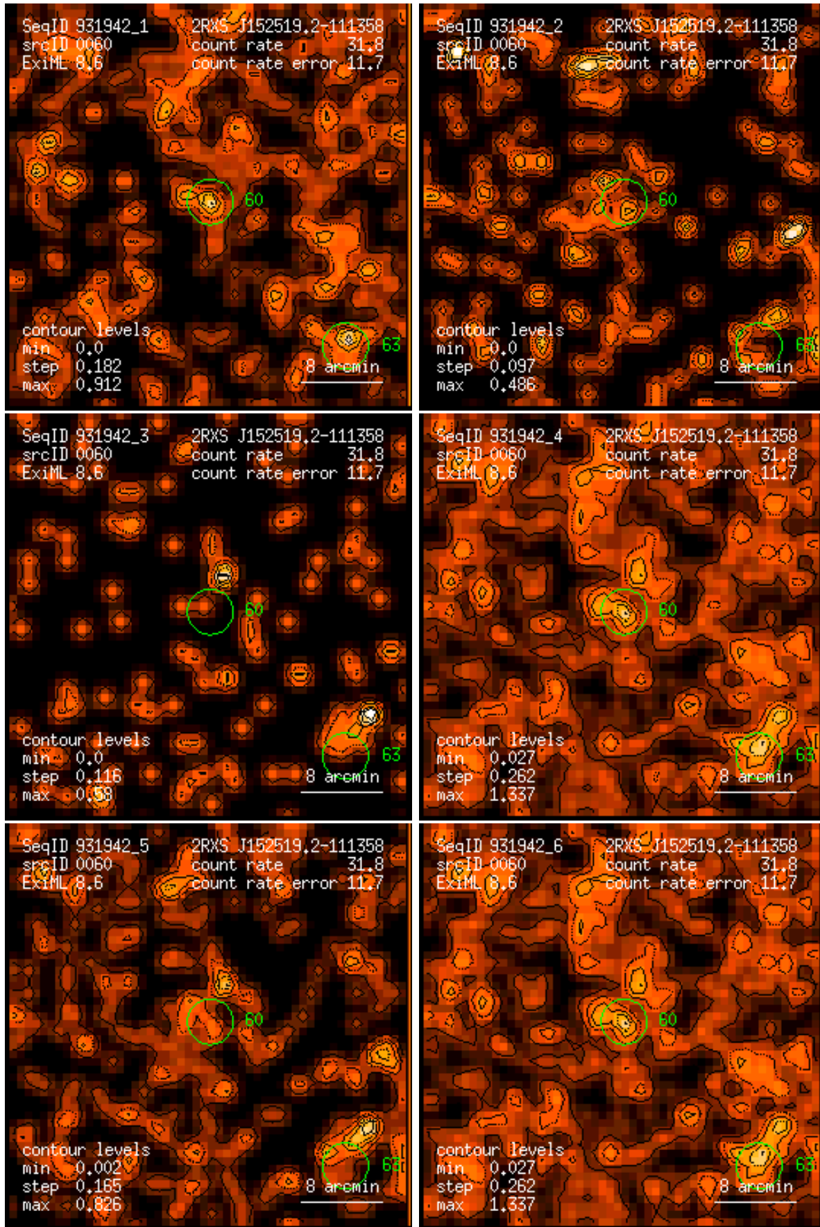
Figure 60: RASS 931942: detection 0060: band rate images, Gaussian filter: (1) PSPC channels 11 – 41, (2) 52 – 90, (3) 91 – 201, (4) 11 – 235, (5) 52 – 201, (6) 11 – 201. Broad band rates in counts/ks. Band rate contour levels in counts/ks/arcmin 2 .
