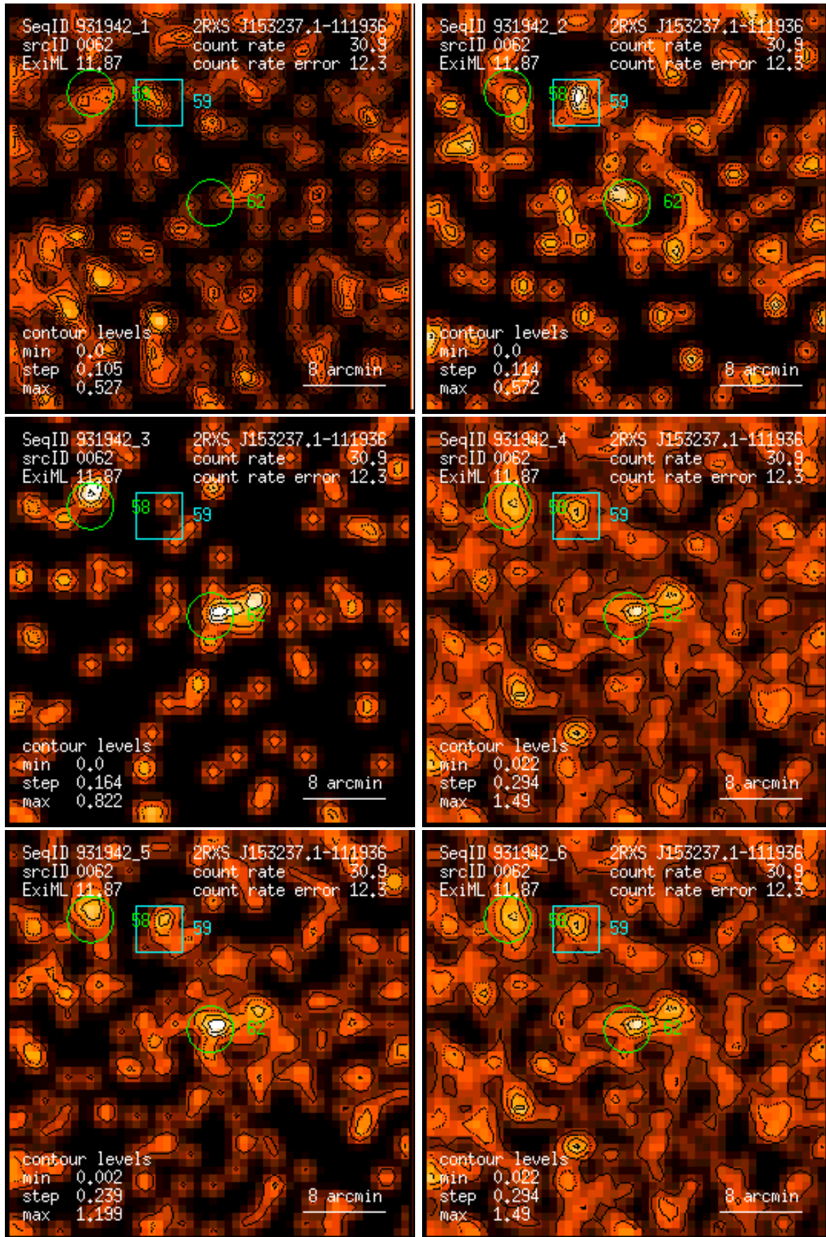
Figure 62: RASS 931942: detection 0062: band rate images, Gaussian filter: (1) PSPC channels 11 – 41, (2) 52 – 90, (3) 91 – 201, (4) 11 – 235, (5) 52 – 201, (6) 11 – 201. Broad band rates in counts/ks. Band rate contour levels in counts/ks/arcmin 2 .
