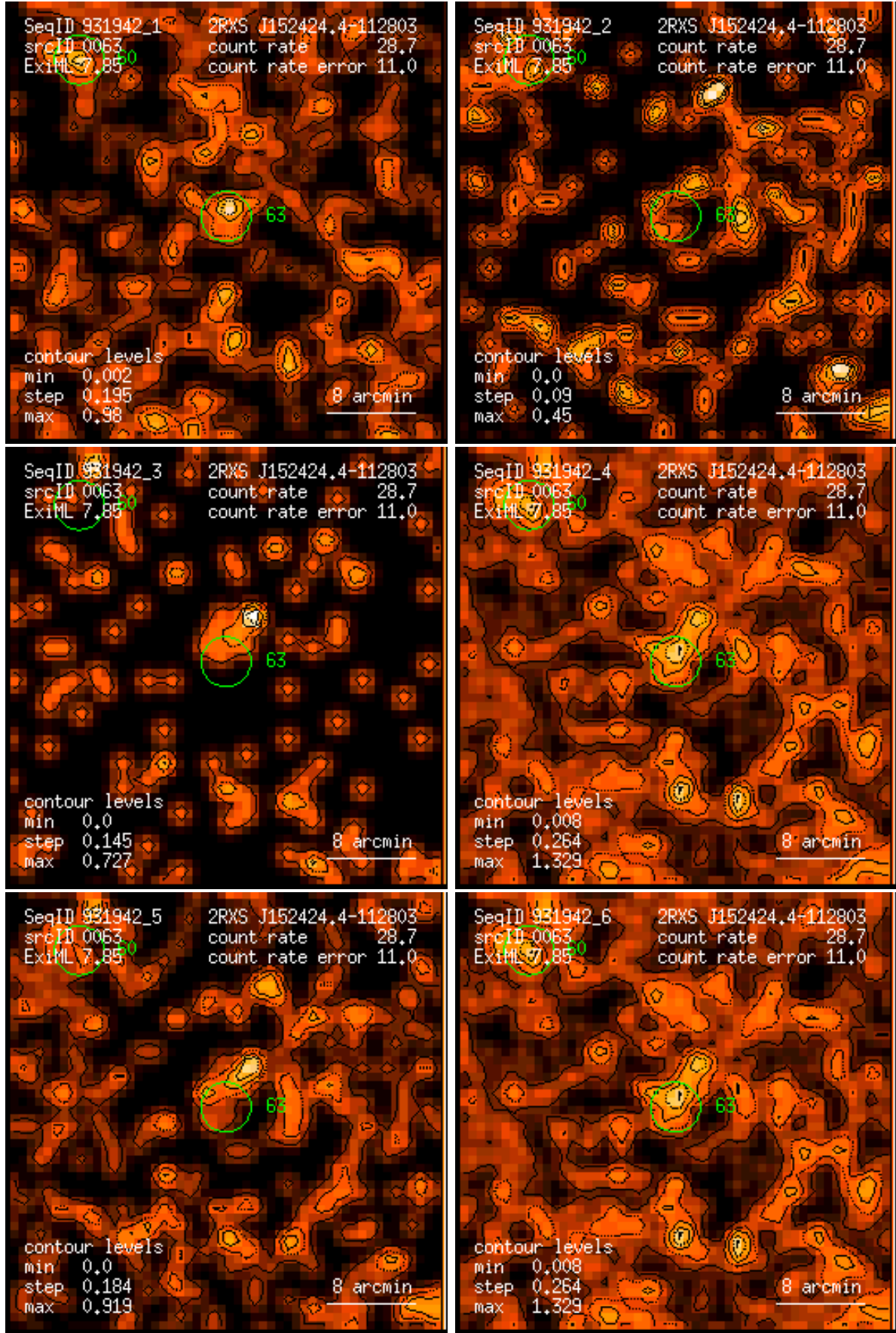
Figure 63: RASS 931942: detection 0063: band rate images, Gaussian filter: (1) PSPC channels 11 – 41, (2) 52 – 90, (3) 91 – 201, (4) 11 – 235, (5) 52 – 201, (6) 11 – 201. Broad band rates in counts/ks. Band rate contour levels in counts/ks/arcmin 2 .
