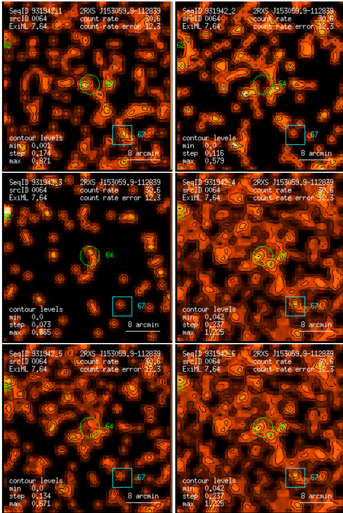
Figure 64: RASS 931942: detection 0064: band rate images, Gaussian filter: (1) PSPC channels 11 – 41, (2) 52 – 90, (3) 91 – 201, (4) 11 – 235, (5) 52 – 201, (6) 11 – 201. Broad band rates in counts/ks. Band rate contour levels in counts/ks/arcmin 2 .
