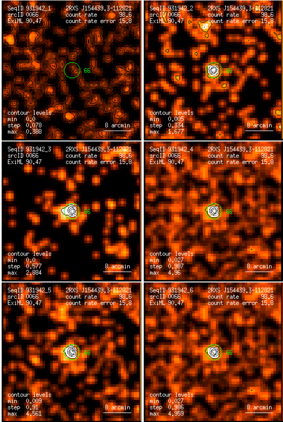
Figure 66: RASS 931942: detection 0066: band rate images, Gaussian filter: (1) PSPC channels 11 – 41, (2) 52 – 90, (3) 91 – 201, (4) 11 – 235, (5) 52 – 201, (6) 11 – 201. Broad band rates in counts/ks. Band rate contour levels in counts/ks/arcmin 2 .
