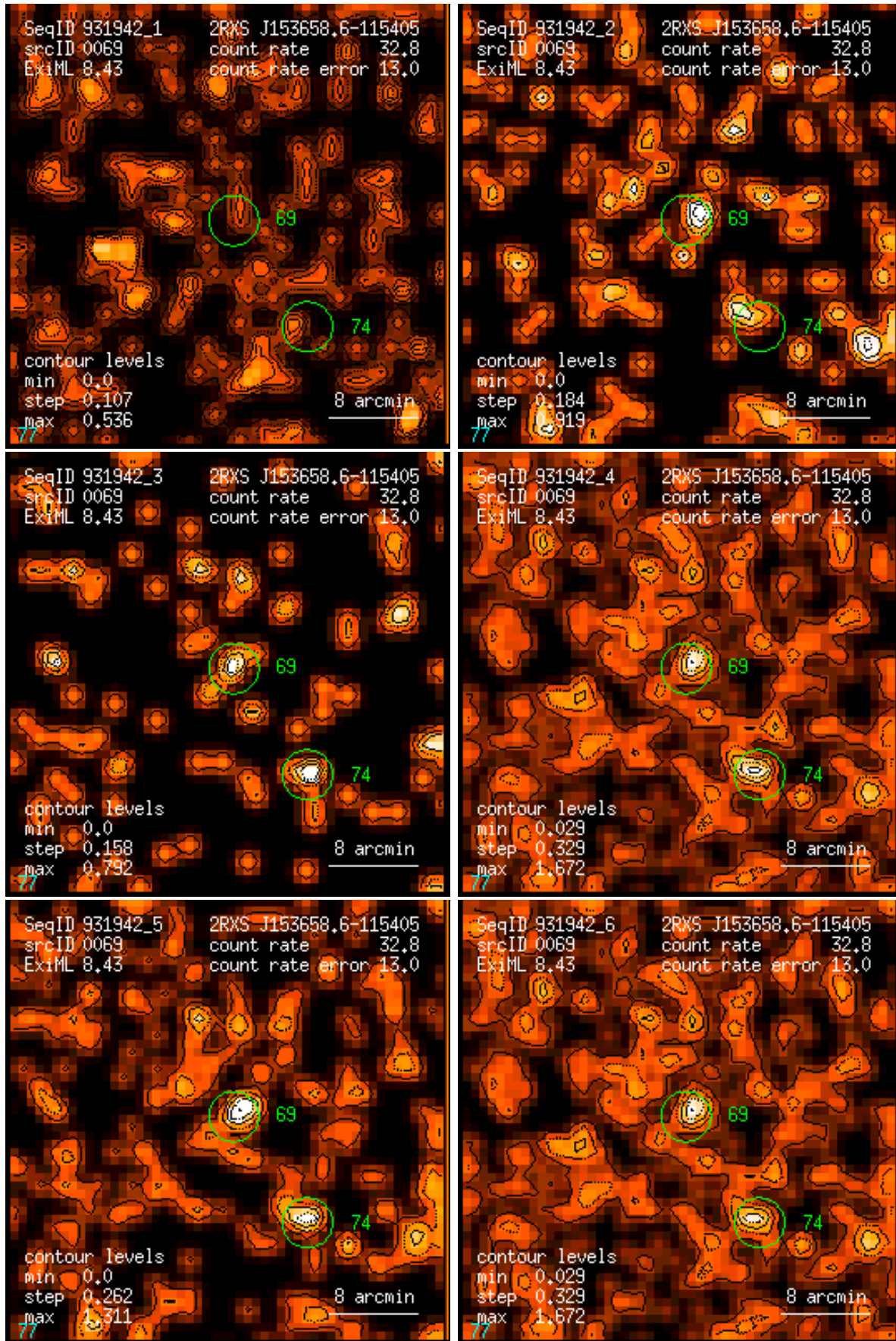
Figure 69: RASS 931942: detection 0069: band rate images, Gaussian filter: (1) PSPC channels 11 – 41, (2) 52 – 90, (3) 91 – 201, (4) 11 – 235, (5) 52 – 201, (6) 11 – 201. Broad band rates in counts/ks. Band rate contour levels in counts/ks/arcmin 2 .
