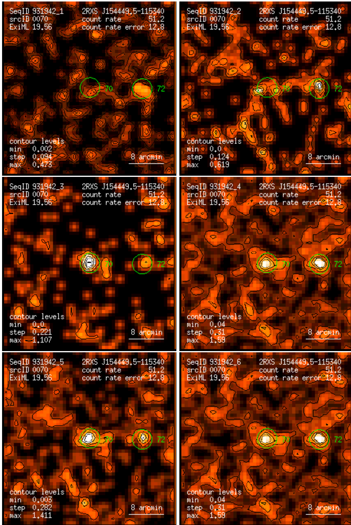
Figure 70: RASS 931942: detection 0070: band rate images, Gaussian filter: (1) PSPC channels 11 – 41, (2) 52 – 90, (3) 91 – 201, (4) 11 – 235, (5) 52 – 201, (6) 11 – 201. Broad band rates in counts/ks. Band rate contour levels in counts/ks/arcmin 2 .
