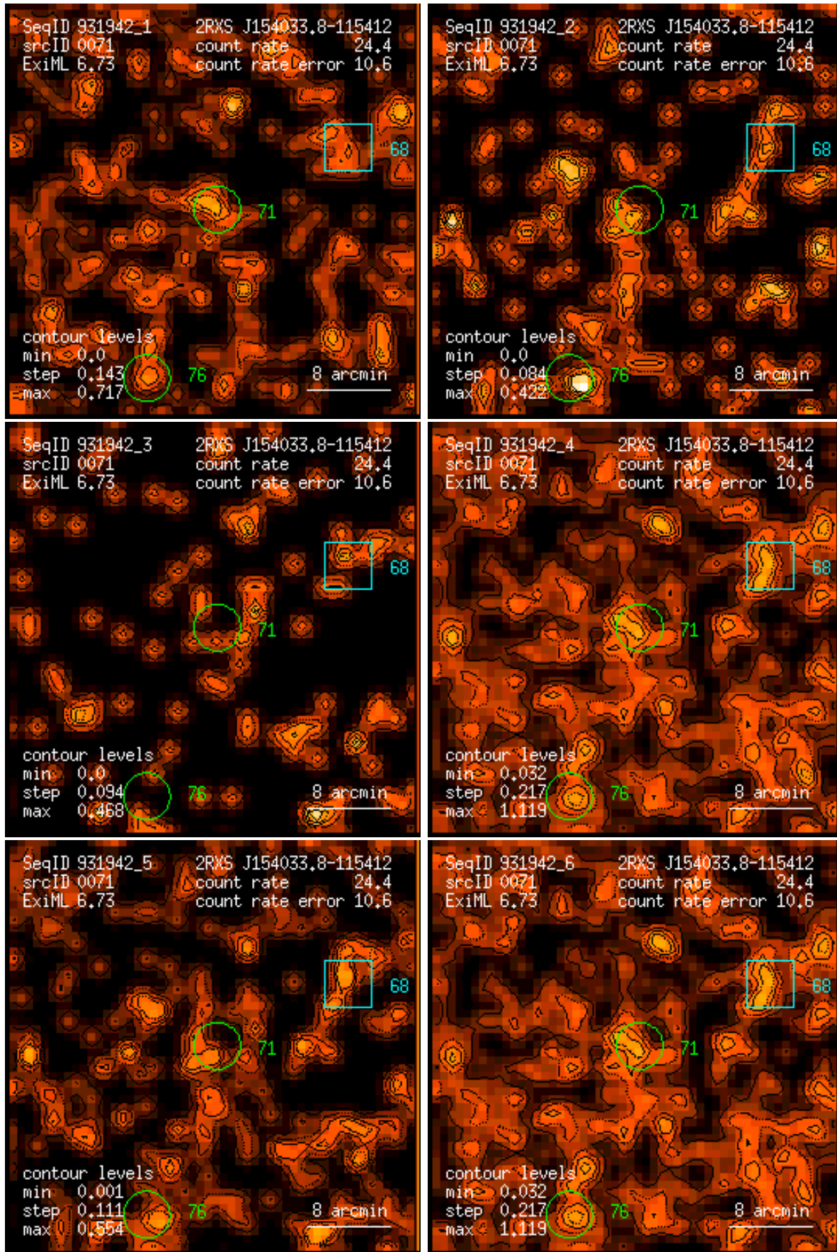
Figure 71: RASS 931942: detection 0071: band rate images, Gaussian filter: (1) PSPC channels 11 – 41, (2) 52 – 90, (3) 91 – 201, (4) 11 – 235, (5) 52 – 201, (6) 11 – 201. Broad band rates in counts/ks. Band rate contour levels in counts/ks/arcmin 2 .
