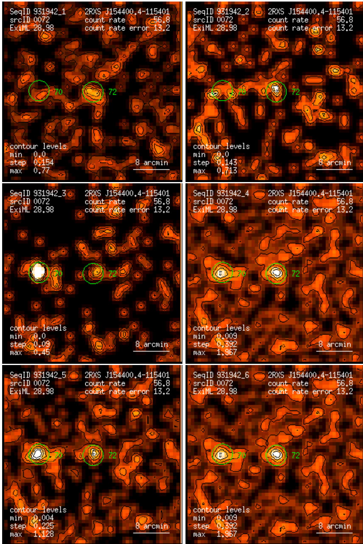
Figure 72: RASS 931942: detection 0072: band rate images, Gaussian filter: (1) PSPC channels 11 – 41, (2) 52 – 90, (3) 91 – 201, (4) 11 – 235, (5) 52 – 201, (6) 11 – 201. Broad band rates in counts/ks. Band rate contour levels in counts/ks/arcmin 2 .
