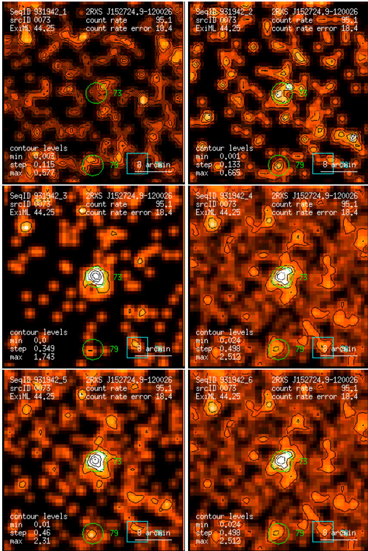
Figure 73: RASS 931942: detection 0073: band rate images, Gaussian filter: (1) PSPC channels 11 – 41, (2) 52 – 90, (3) 91 – 201, (4) 11 – 235, (5) 52 – 201, (6) 11 – 201. Broad band rates in counts/ks. Band rate contour levels in counts/ks/arcmin 2 .
