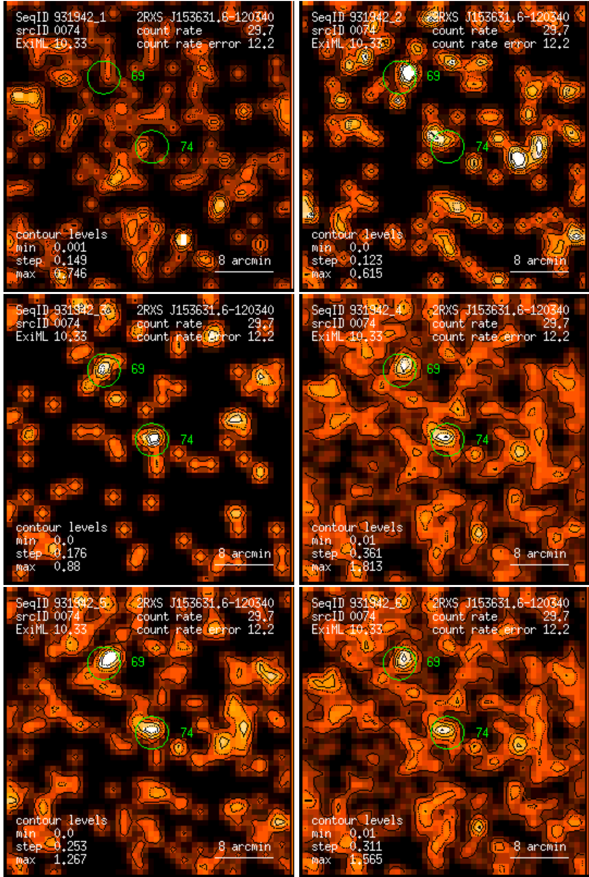
Figure 74: RASS 931942: detection 0074: band rate images, Gaussian filter: (1) PSPC channels 11 – 41, (2) 52 – 90, (3) 91 – 201, (4) 11 – 235, (5) 52 – 201, (6) 11 – 201. Broad band rates in counts/ks. Band rate contour levels in counts/ks/arcmin 2 .
